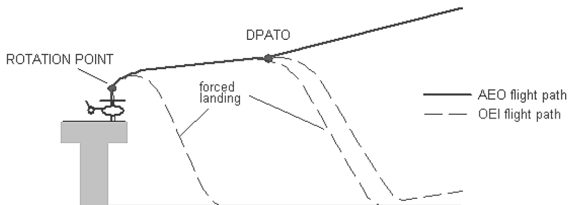
Figure 1: Take-off profile
