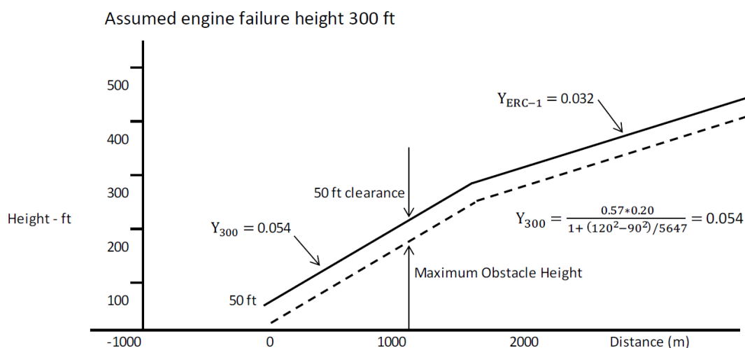
Figure 1: Assumed engine failure height 300 ft
