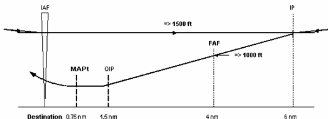
Figure 5: Missed approach area left & right
