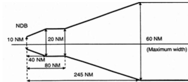
Figure 2: Corridor width from an NDB
