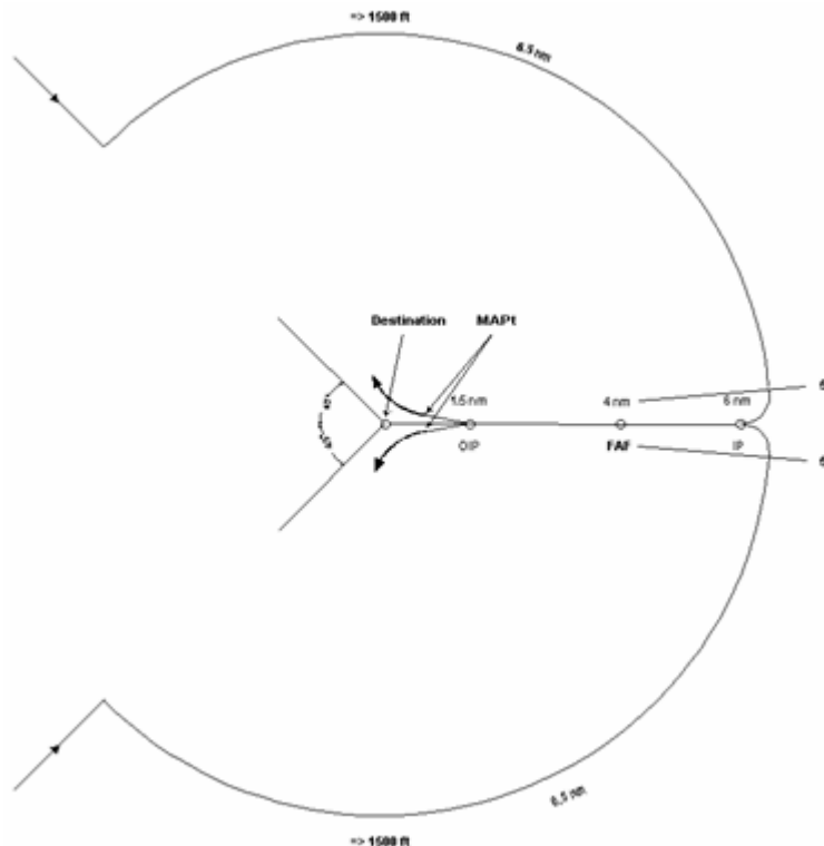
Figure 1: Arc procedure
