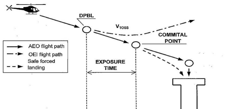
Figure 6: Typical landing profile PC2 to a helideck/elevated FATO with exposure time, non-congested hostile environment
