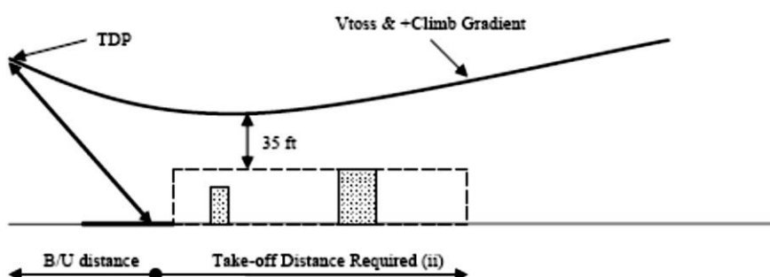
Figure 3: Helipad take – off
