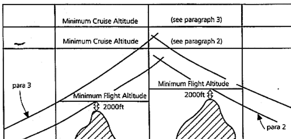
Figure 1: Intersection of the two drift down paths
