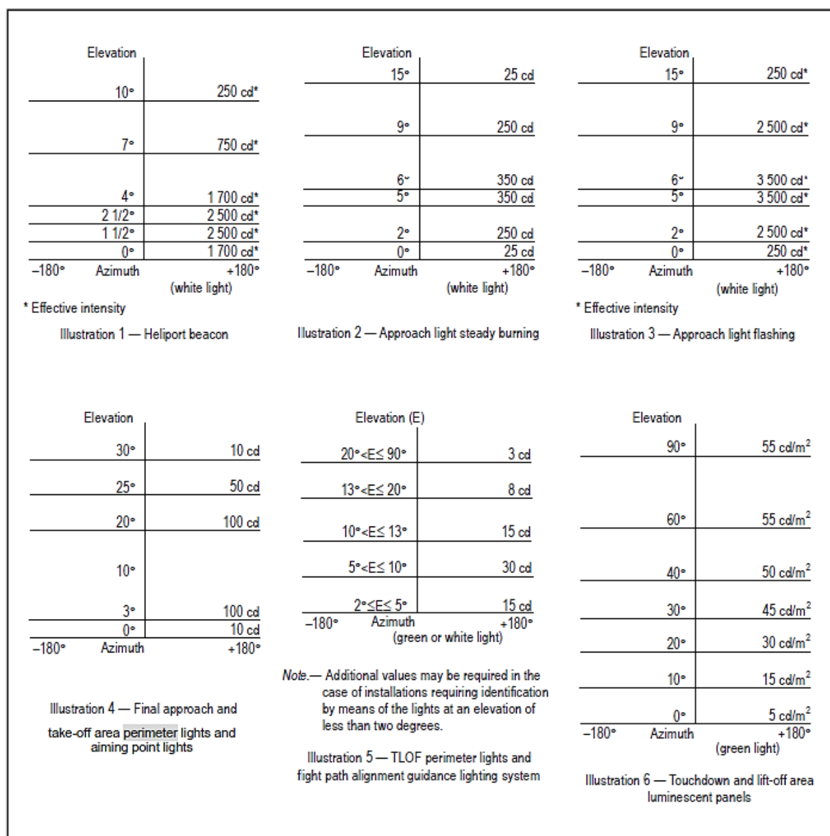
Figure 5-12. Isocandela diagrams
