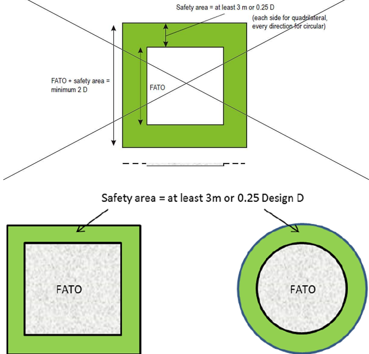
Figure 3-1. FATO and associated safety area
