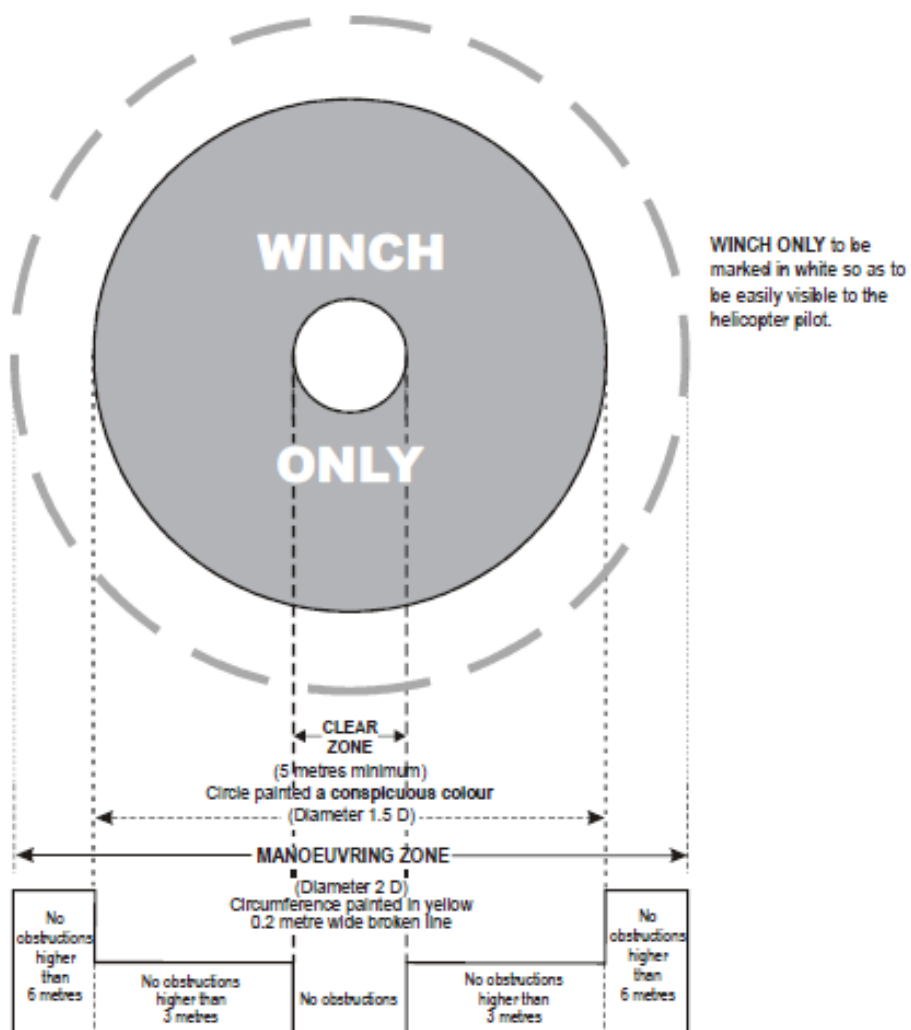
Figure 4-7. Winching area of a ship
