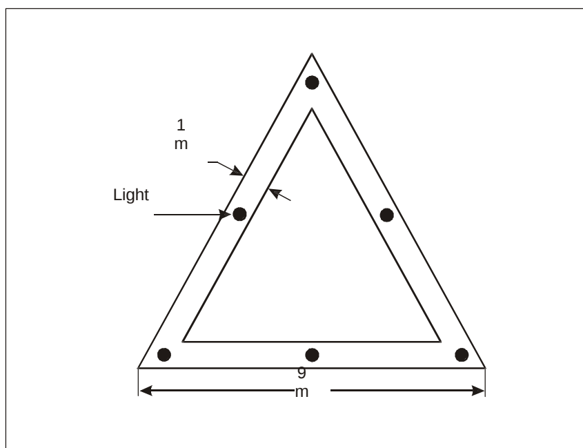
Figure 24. Aiming point marking (ICAO Annex 14 Vol II, Fig 5-6)
