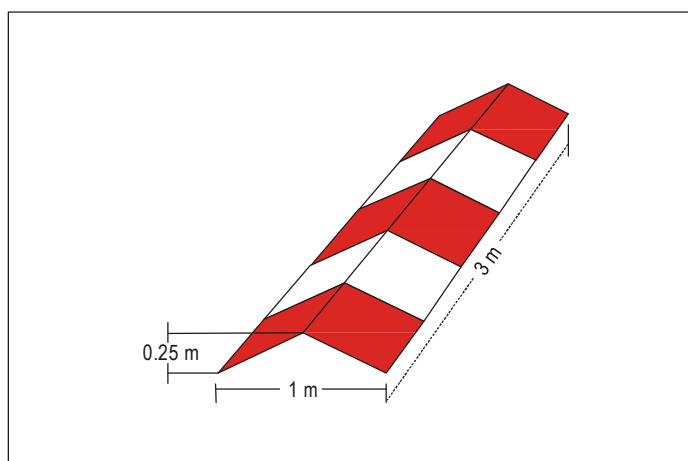
Figure 23. Runway-type FATO edge marker (ICAO Annex 14, Vol II, Fig. 5-5)
