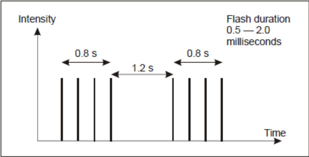
Figure 5-11. Heliport beacon flash characteristics
