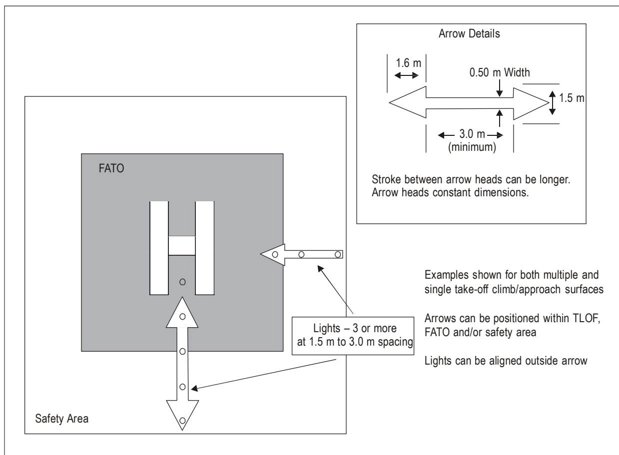
Figure 27. Flight path alignment guidance markings and lights (ICAO Annex 14, Vol II, Fig 5-9)
