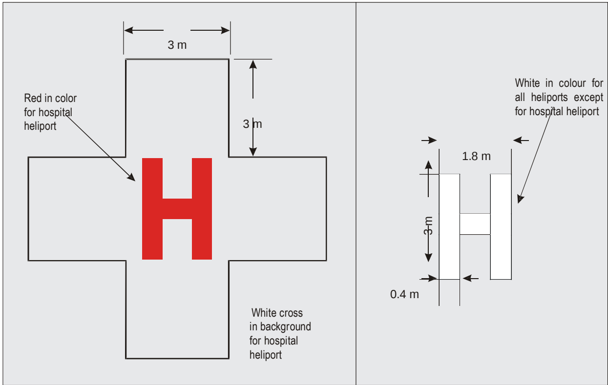
Figure 21. Hospital heliport identification and heliport identification marking (ICAO Annex 14, Vol. II, Fig. 5-3)
