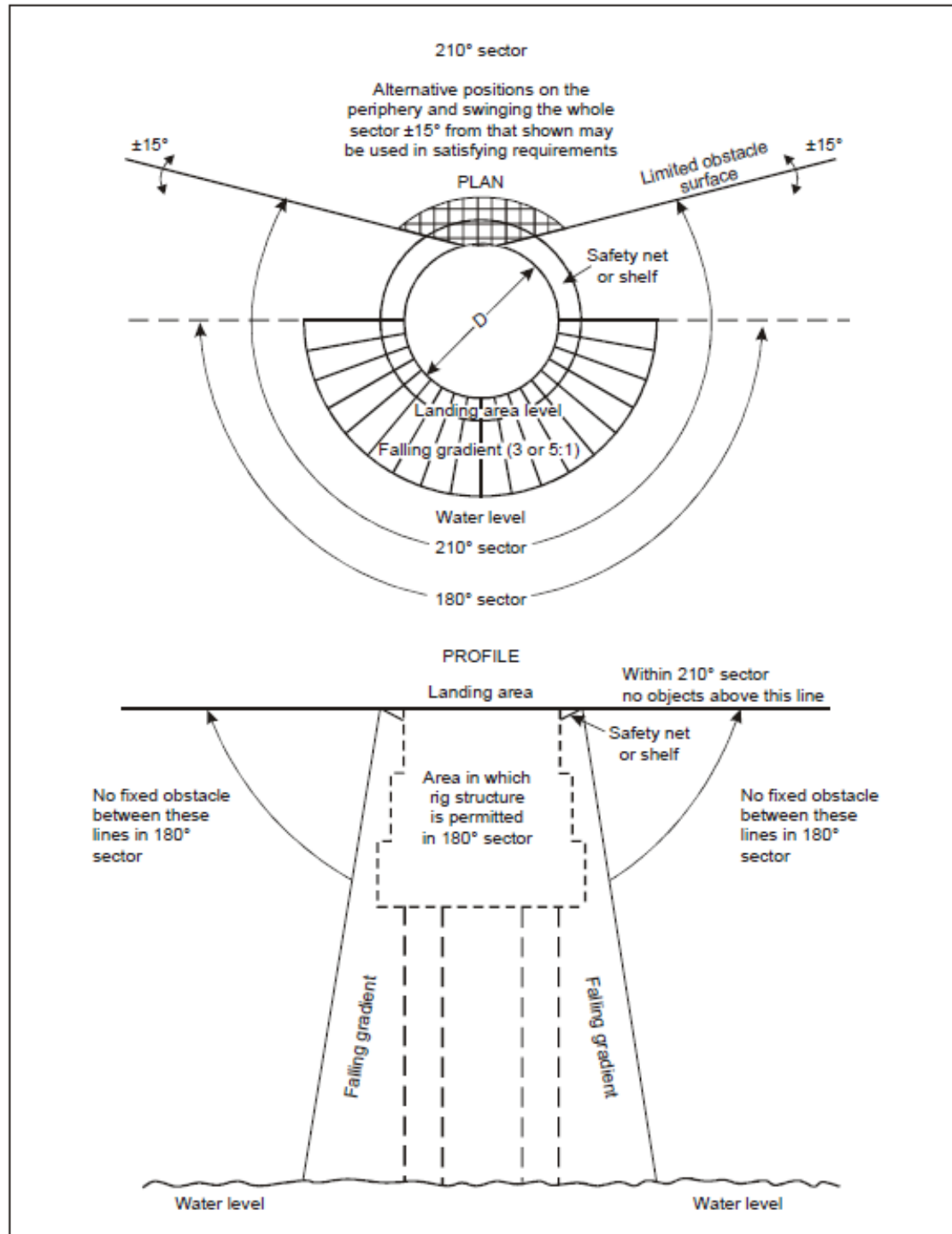
Figure 4-2. Helideck obstacle-free sector
