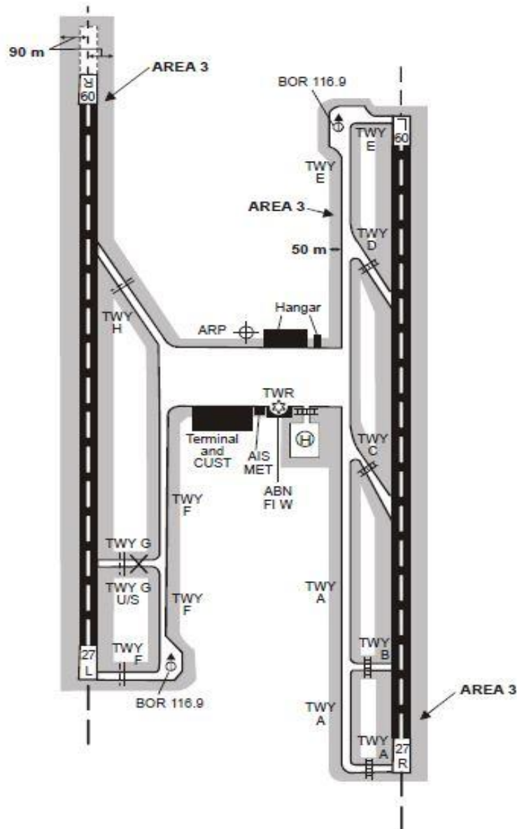
Figure A8-3. Terrain and obstacle data collection surface — Area 3
