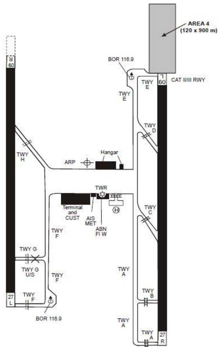
Figure A8-4. Terrain and obstacle data collection surface — Area 4
