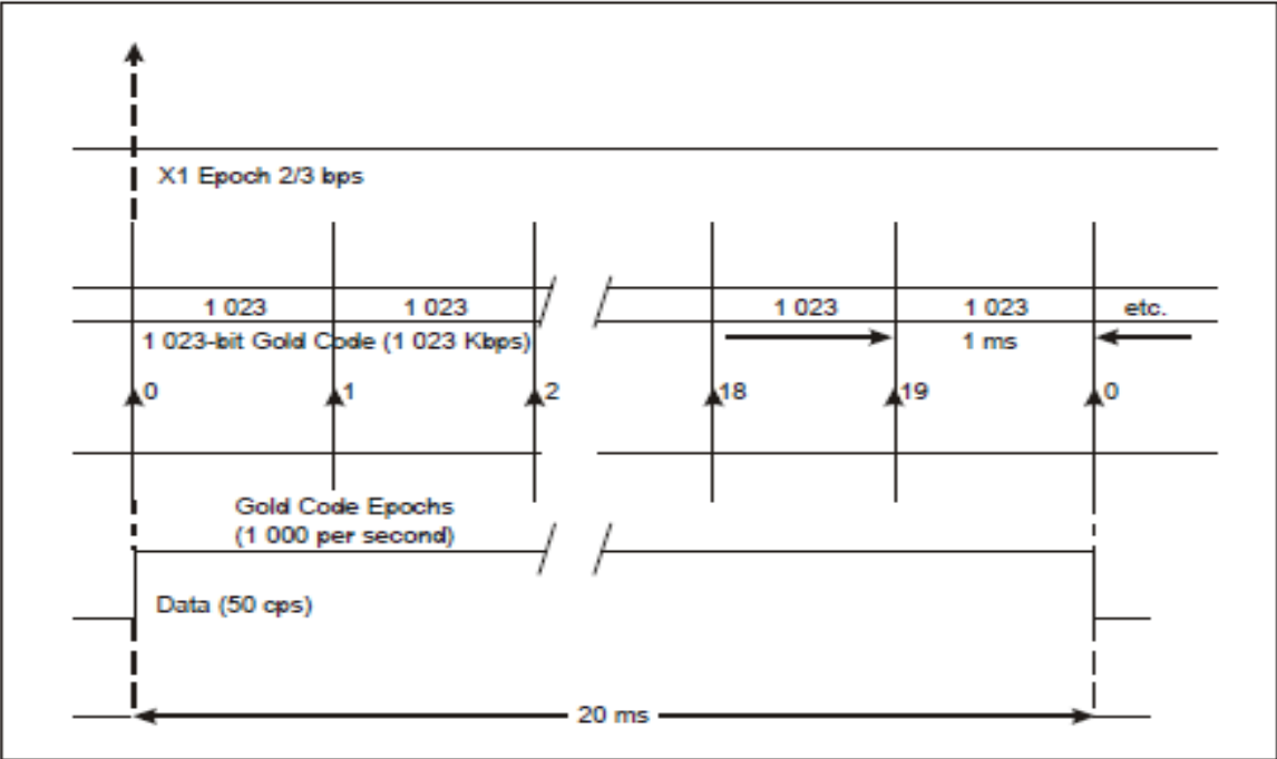
Figure B-1. C/A code timing relationships
