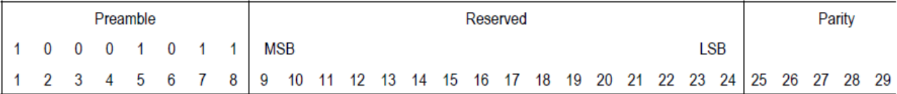
Figure B-3. TLM word format
