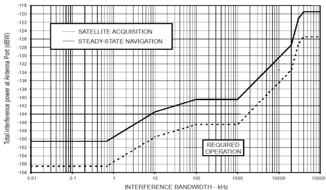
Figure B-17. Interference thresholds versus bandwidth for GPS L1 and SBAS L1 receivers
