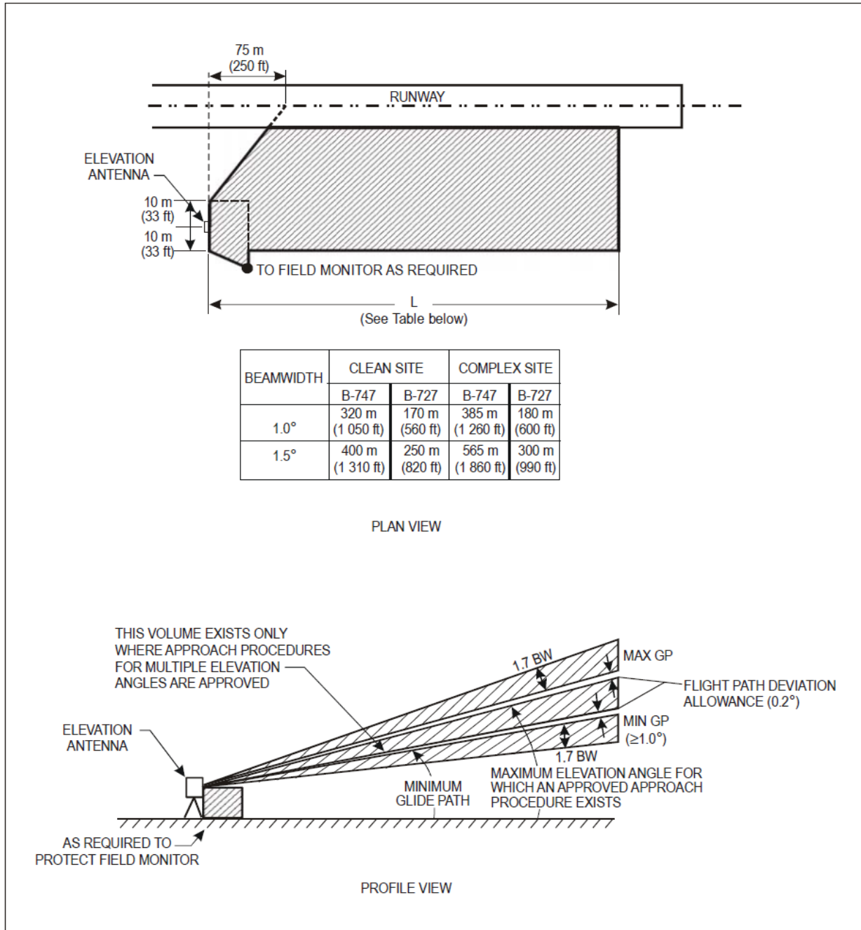
Figure G-24. Typical elevation critical and sensitive areas/volume
