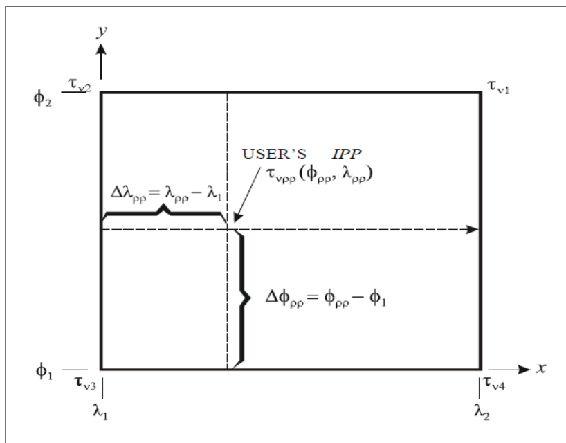
Figure B-13. IGP numbering convention (four IGPs)
