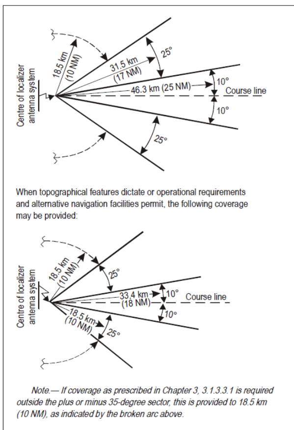
Figure C-7A. Localizer coverage with respect to azimuth
