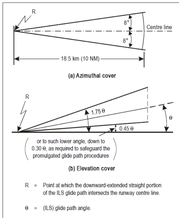
Figure 10. Glide path coverage
