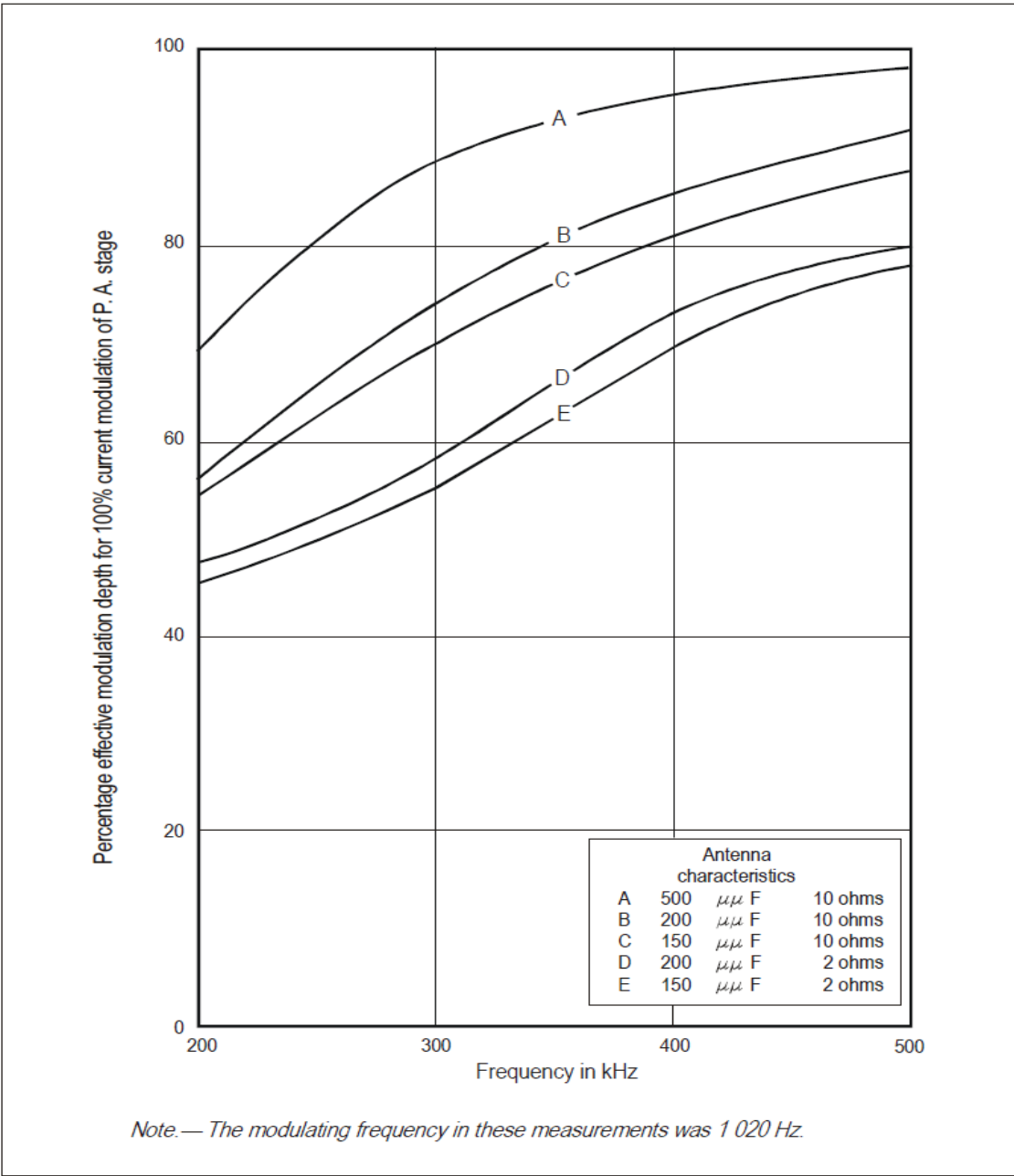
Figure C-19. The effect of antenna Q on the depth of modulation of the radiated signal
