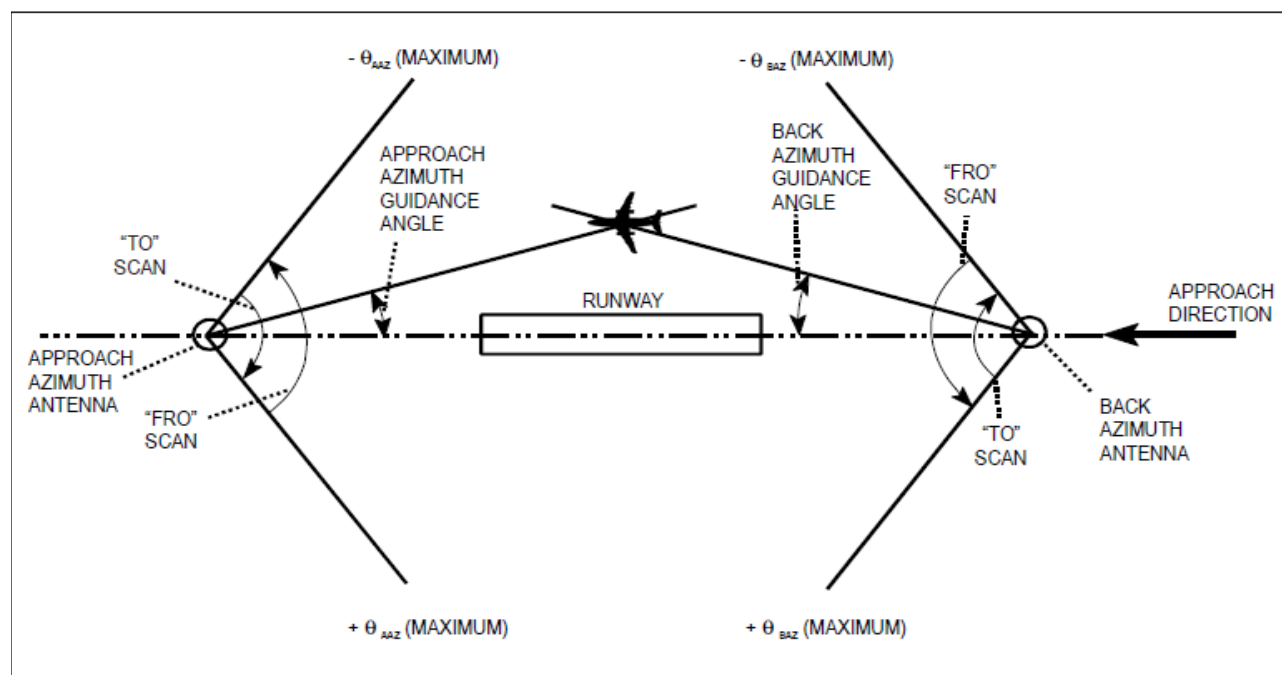
Figure G-4. Scanning conventions for azimuth guidance functions
