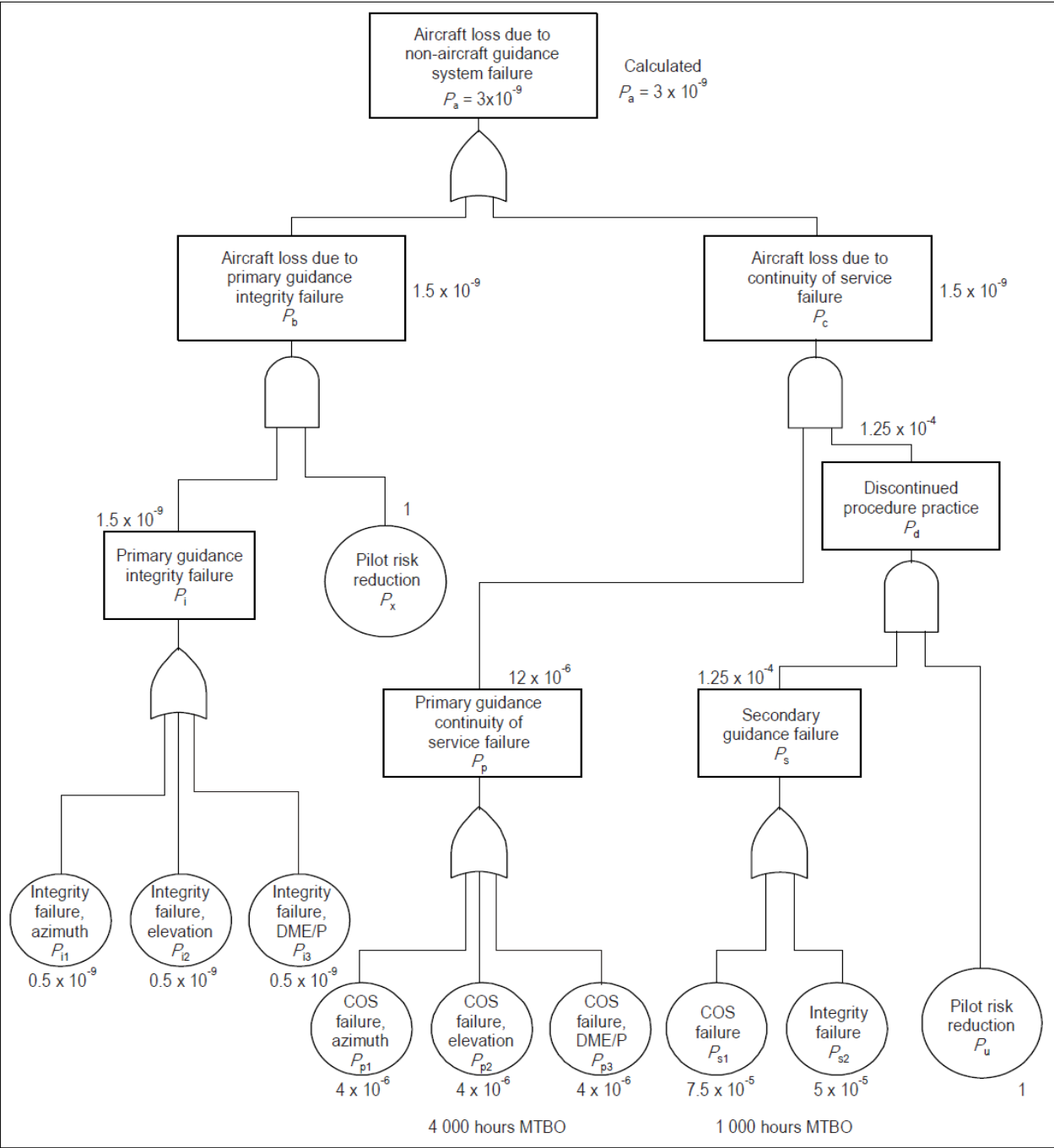
Figure A-3. MLS/RNAV obstacle rich risk tree
