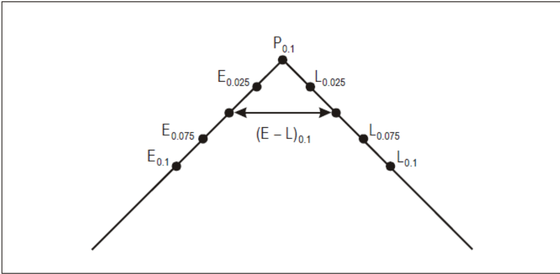
Figure D-18. “Close-in” correlation peak and measured correlator values
