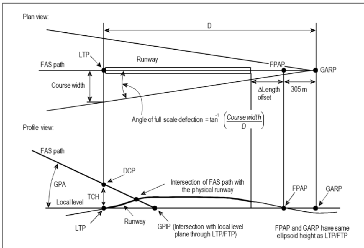
Figure D-15 FAS path definition
