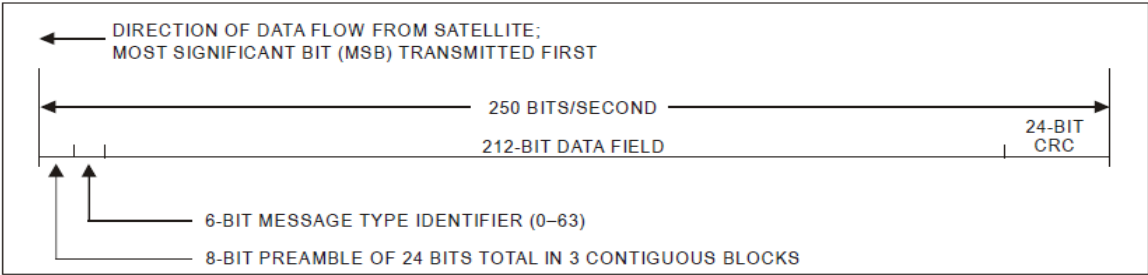
Figure B-12. Data block format
