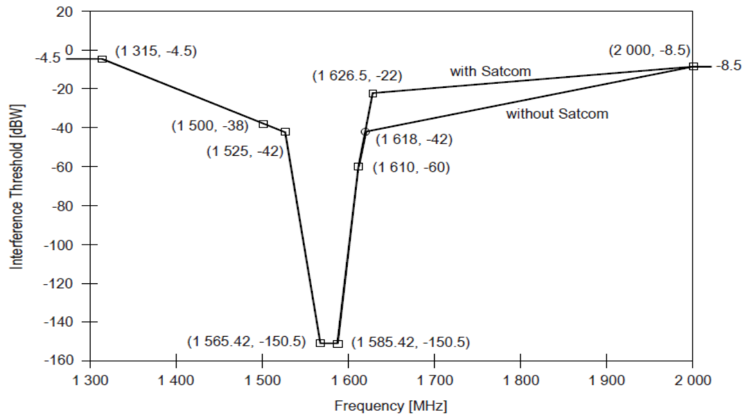
Figure B-15. CW interference thresholds for GPS L1 and SBAS L1 receivers in steady-state navigation
