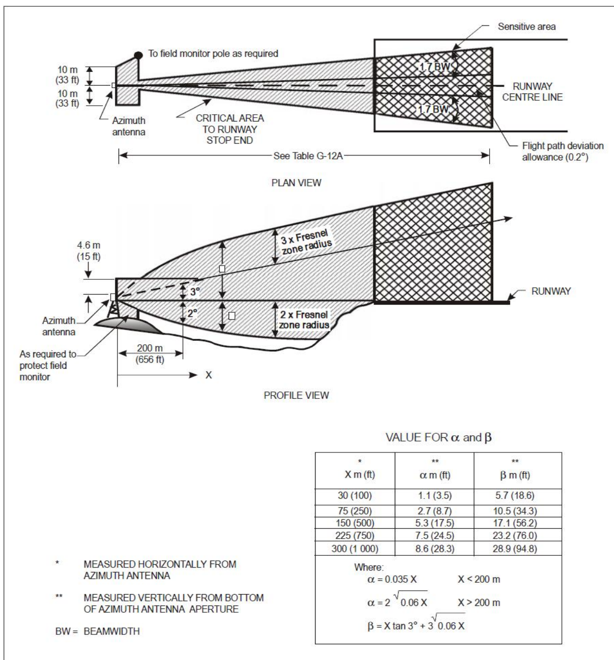
Figure G-23A. Typical azimuth critical and sensitive areas
