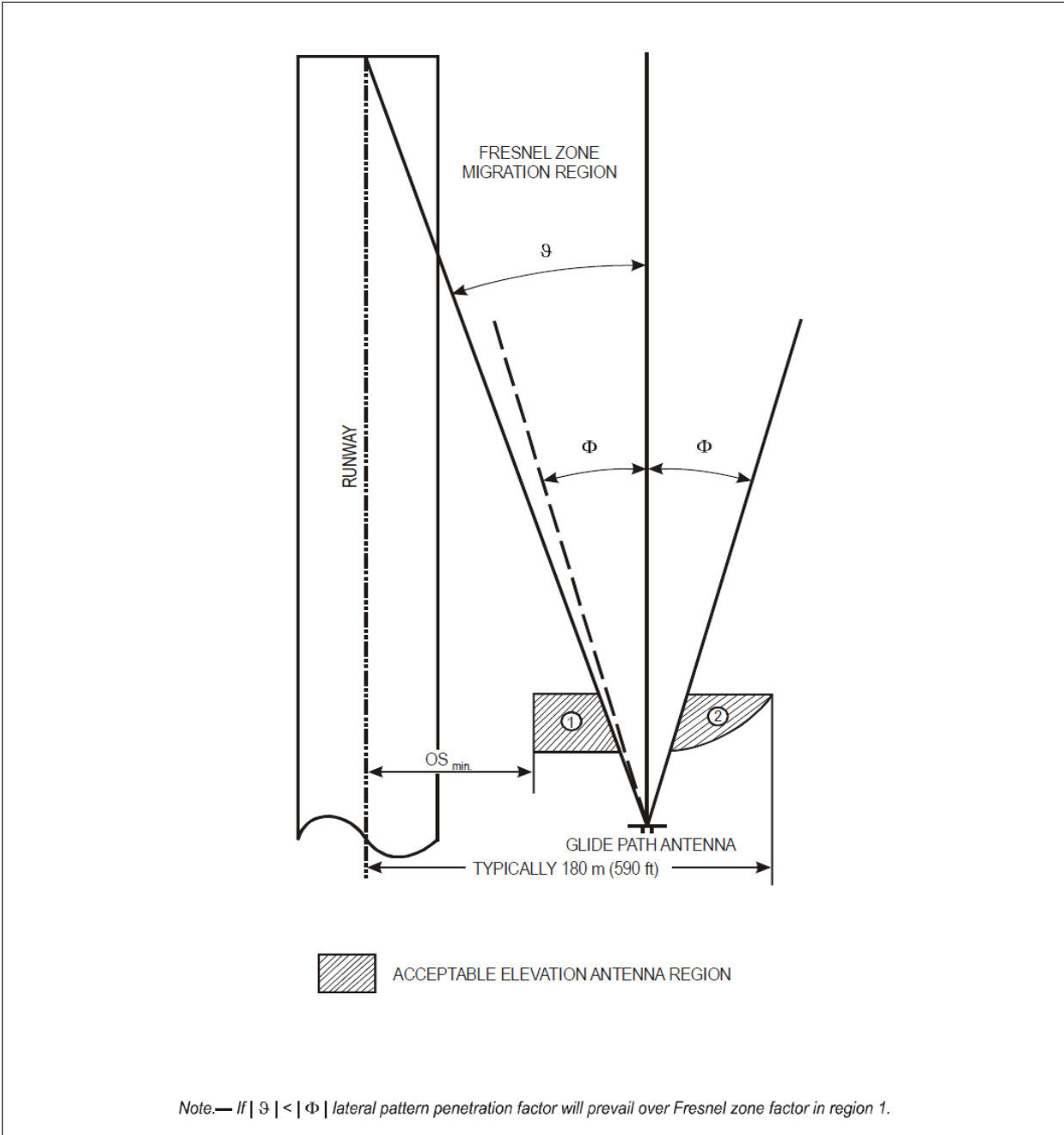
Figure G-18. Elevation antenna regions for collocation with ILS (3° minimum glide path)
