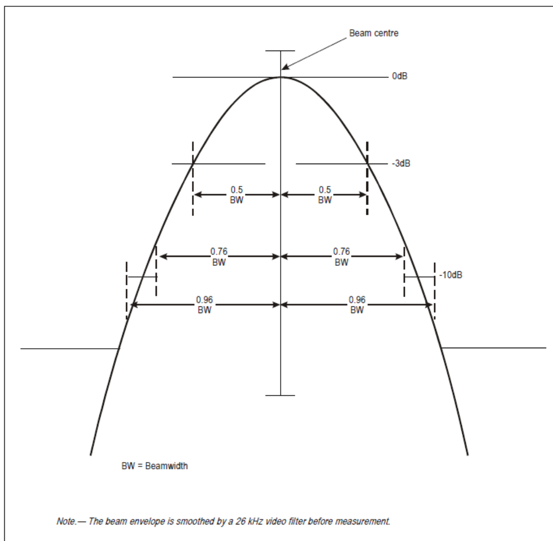
Figure G-16. Far field dynamic signal-in-space
