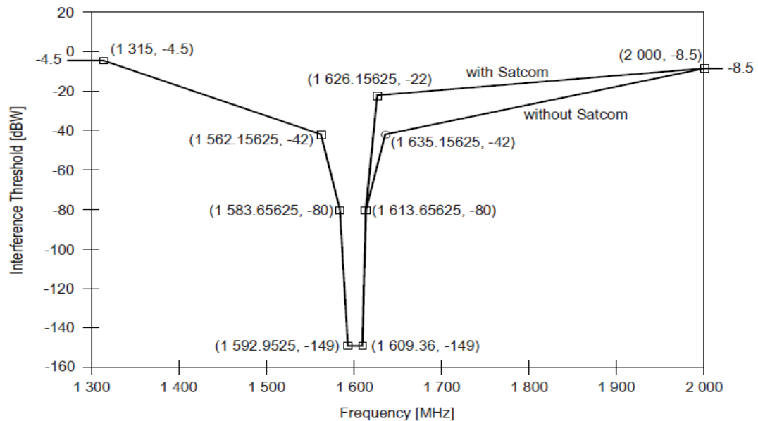
Figure B-16. CW interference thresholds for GLONASS FDMA signals receivers in L1 band in steady-state navigation
