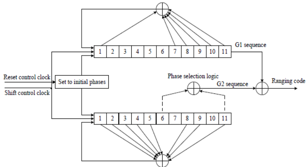
Figure B BDS-1. Generator of C_{B1I}
