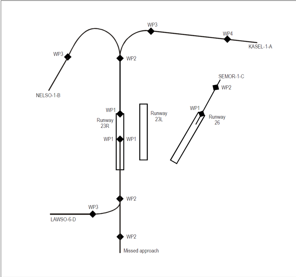
Figure G-15. Diagram of sample MLS/RNAV procedures
