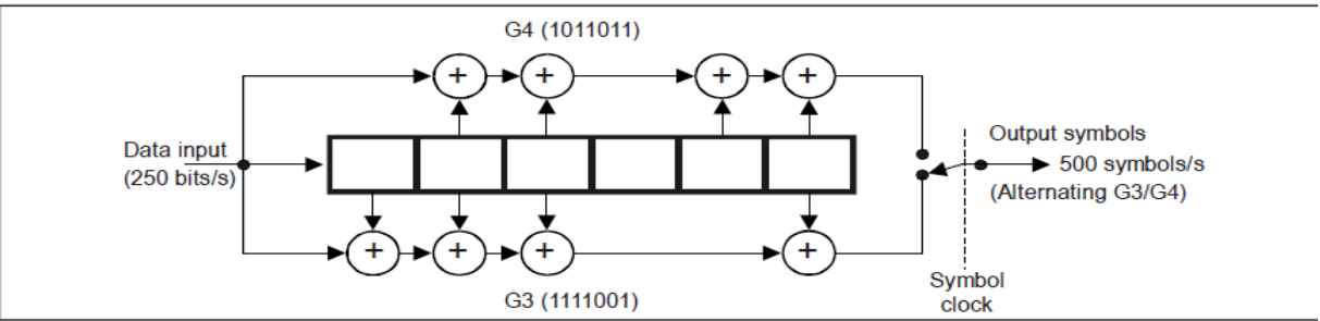
Figure B-11. Convolutional encoding
