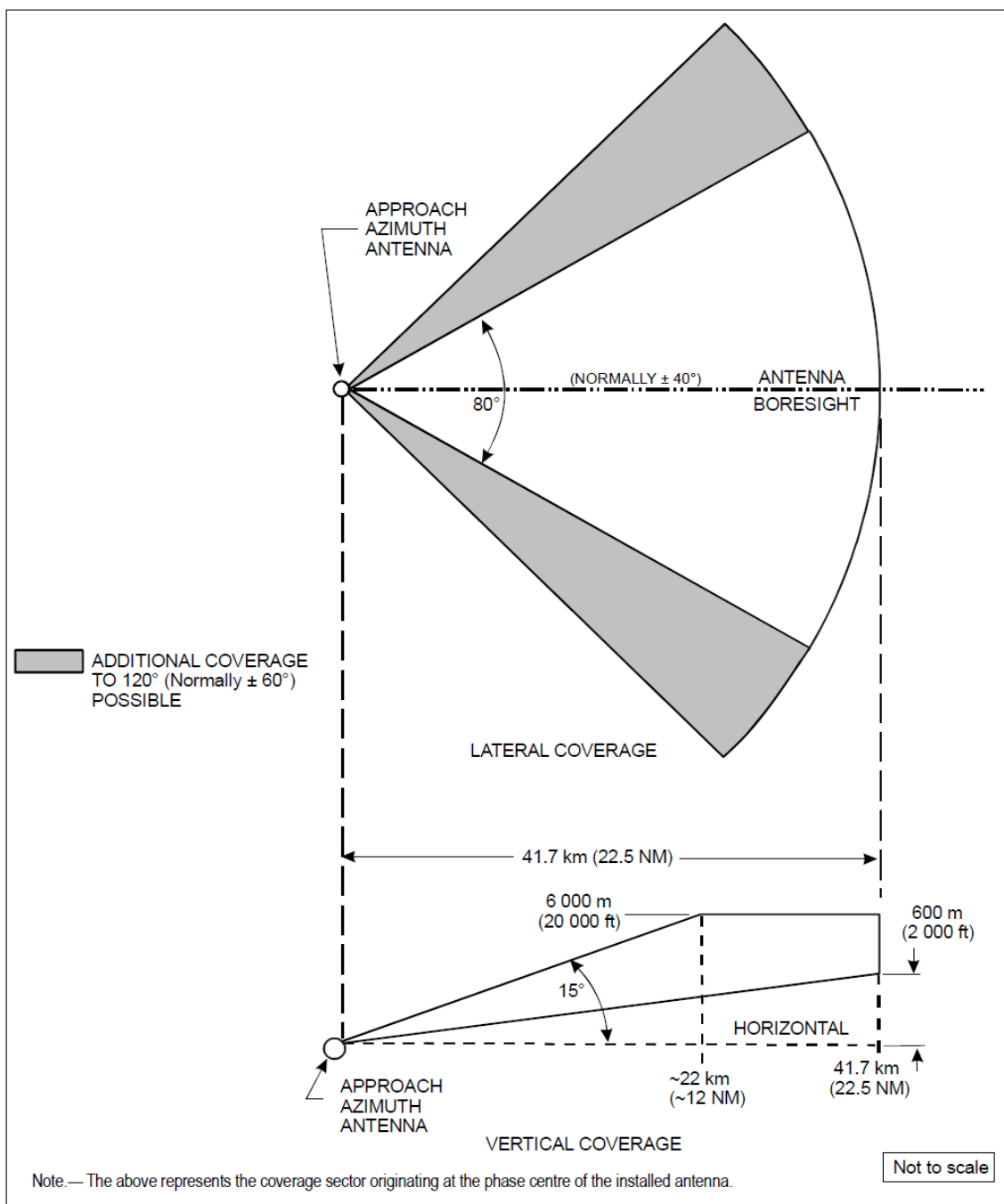
Figure G-5A. Approach azimuth region coverage
