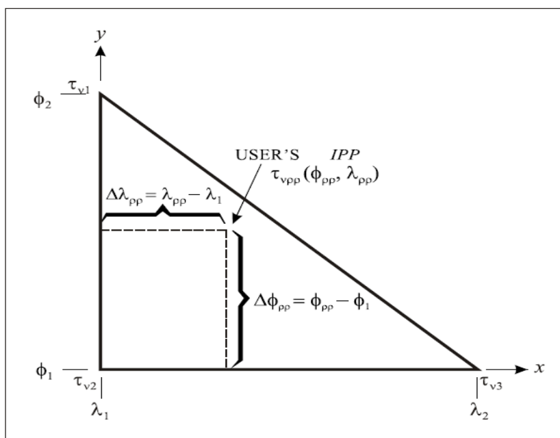
Figure B-14. IGP numbering convention (three IGPs)
