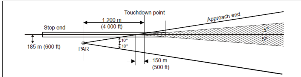
Figure C-15. Minimum set-back of PAR with respect to touchdown for offset of 185 m (600 ft) when aligned to scan plus or minus 10 degrees on QDR of runway
