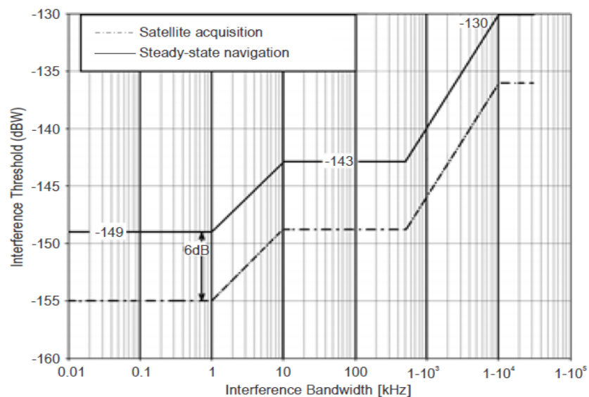
Figure B-17. Interference thresholds versus bandwidth for GPS L1 and SBAS L1 receivers
