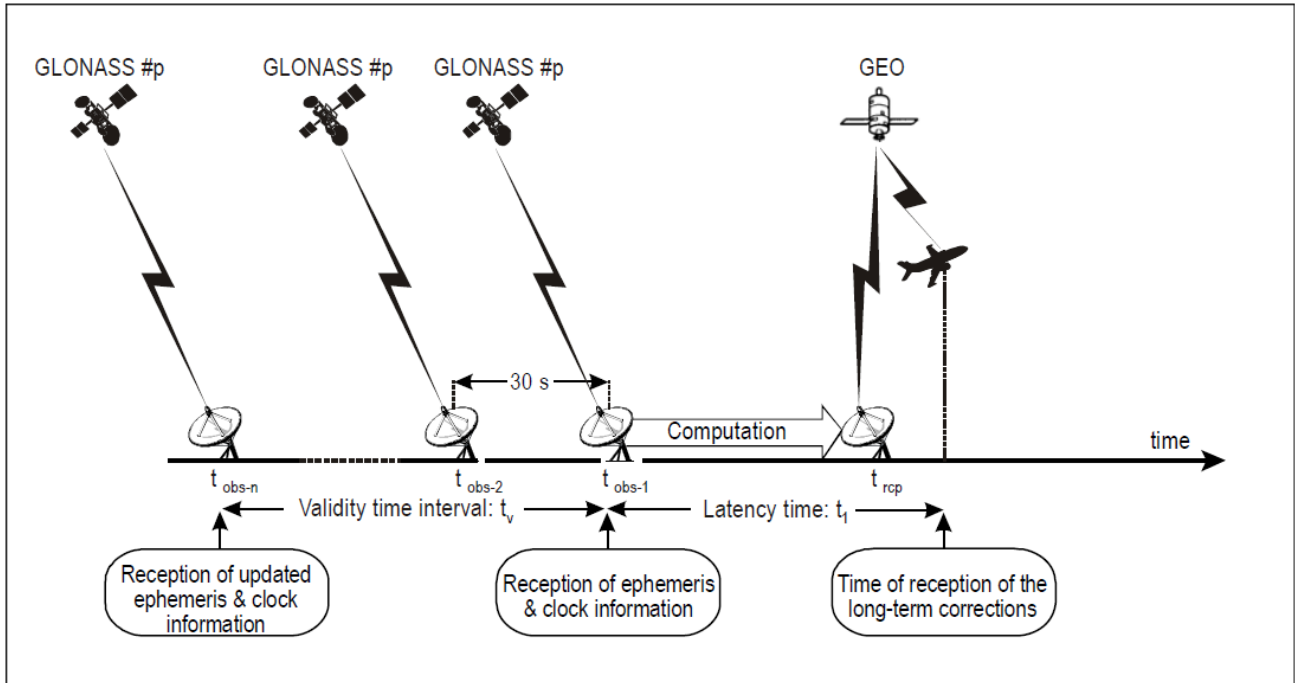
Figure D-3. GLONASS time
