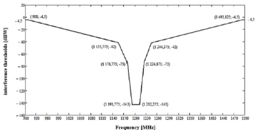
Figure FIG-02. CW interference thresholds for GLONASS CDMA signals receivers in L3 band in steady-state navigation
