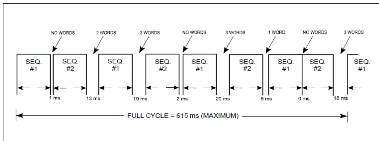
Figure G-3C. Complete multiplex transmission cycle showing open time periods available for data words
