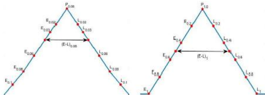
Figure FIG-09. Correlator outputs for Galileo E1-C or BDS B1C_pilot (left) and Galileo E5a-Q or BDS B2a_pilot (right)
