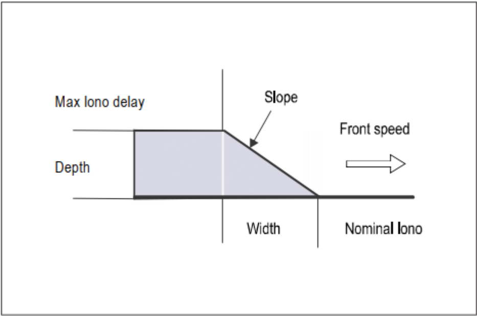
Figure D-7. Moving wedge ionospheric anomaly model
