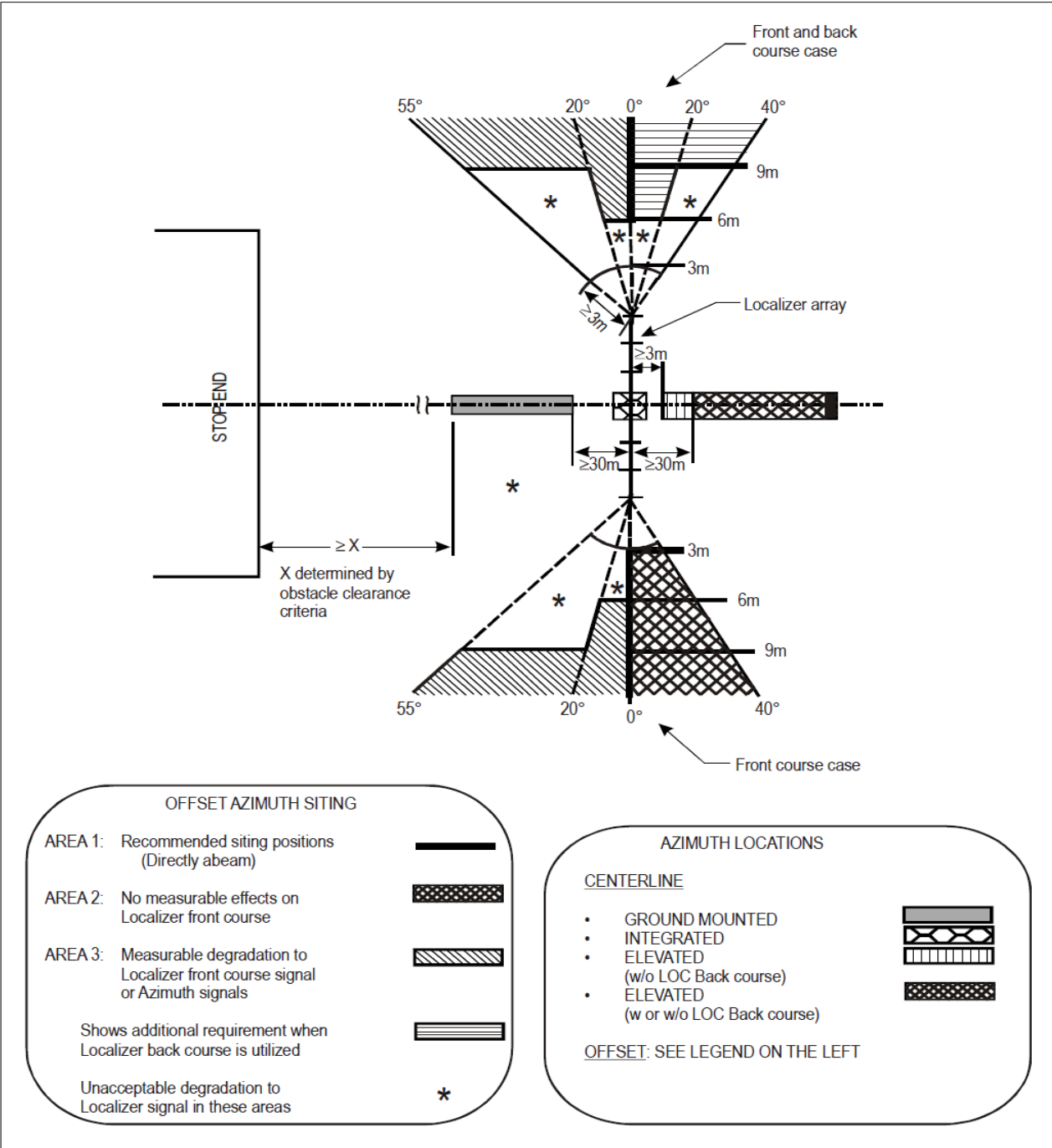
Figure G-21. Azimuth antenna regions for collocation with ILS
