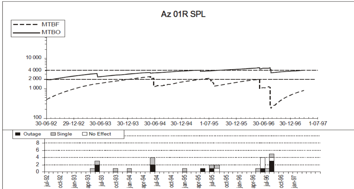
Figure G-35A. Example outage record for MLS azimuth facility
