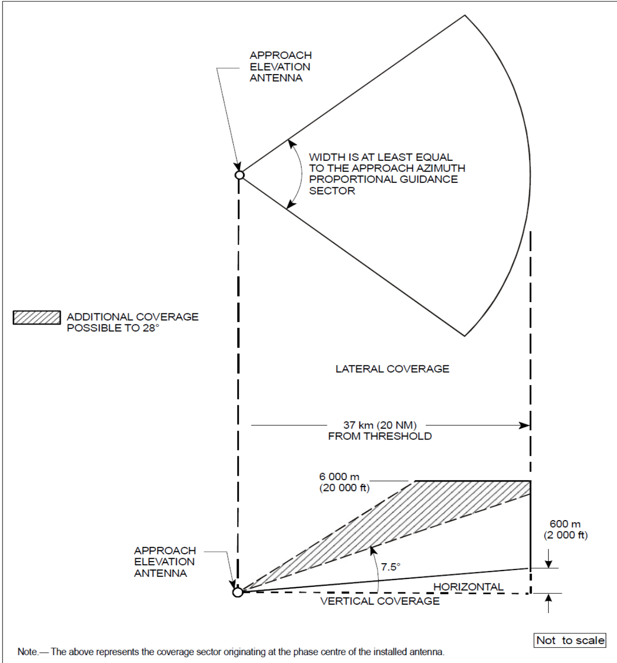
Figure G-10A. Elevation approach region coverage
