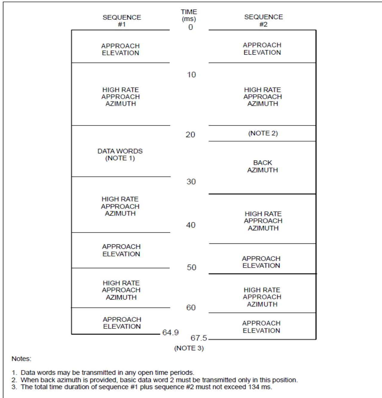
Figure G-3B. Transmission sequence pair which provides for the MLS high rate approach azimuth angle guidance function
