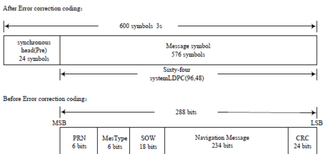
Figure B BDS-5. B-CNAV2 basic frame structure
