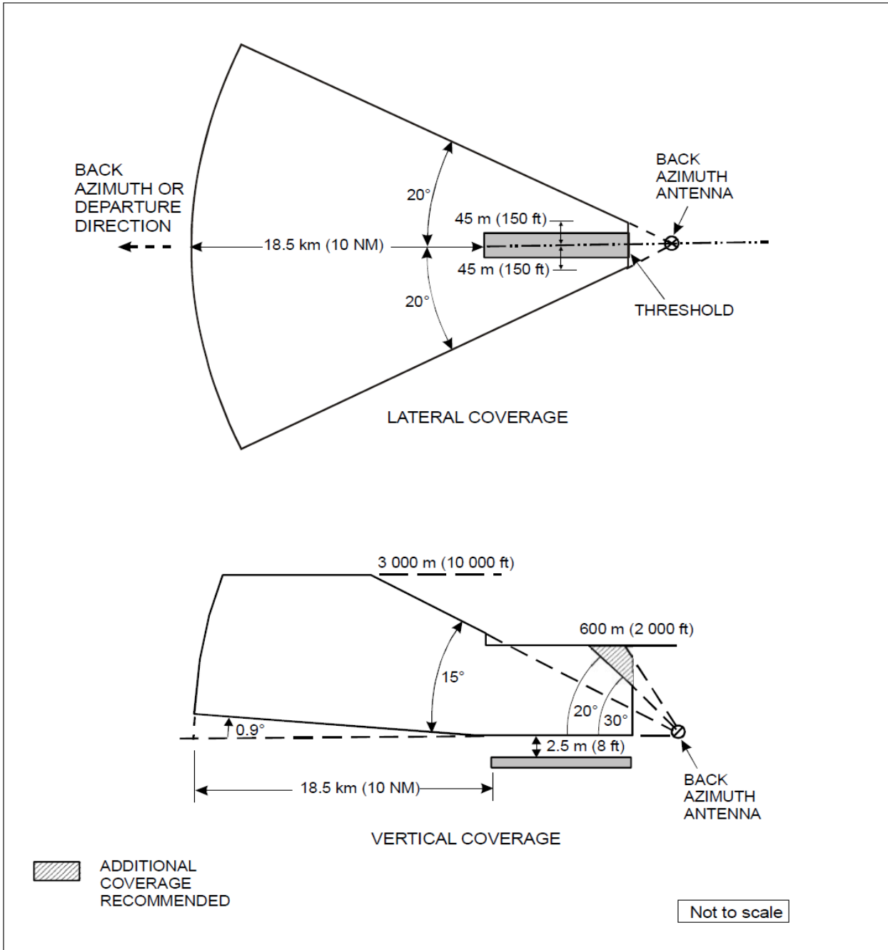
Figure G-6. Back azimuth region coverage
