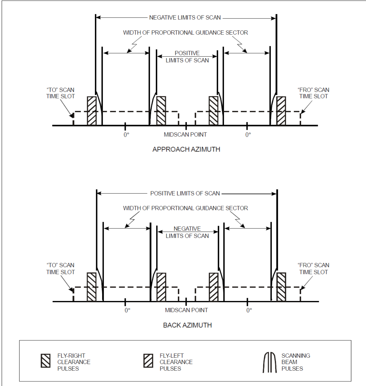
Figure G-7. Clearance pulse conventions for azimuth functions
