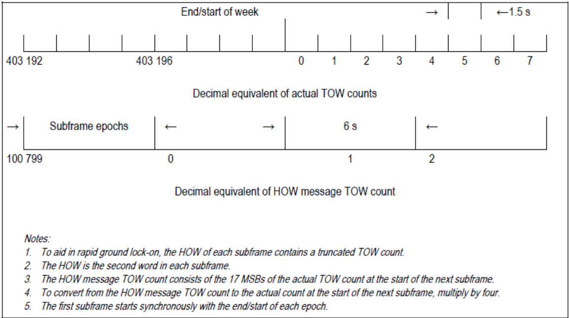
Figure B-5. Time line relationship of HOW
