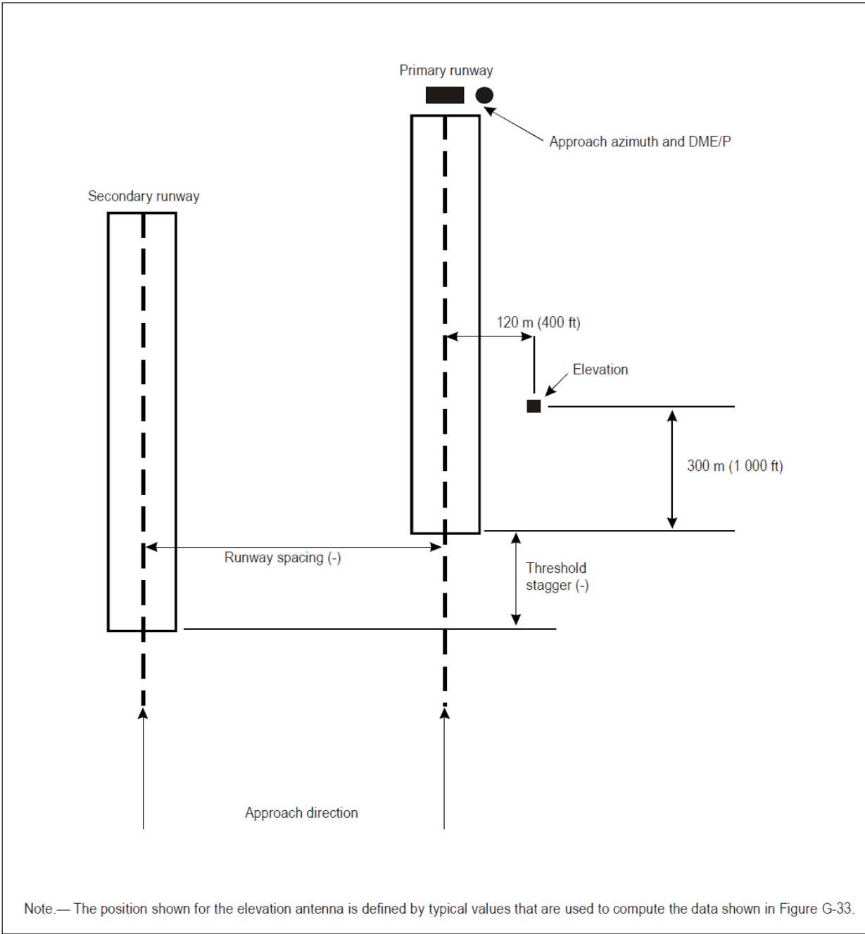
Figure G-32. Runway and equipment geometry for computed centre line approaches to parallel secondary runways
