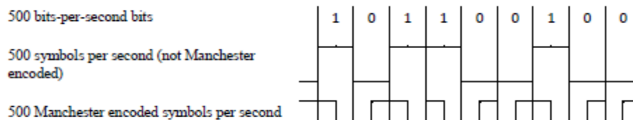
Figure D-19. Bi-binary (Manchester) encoding scheme
