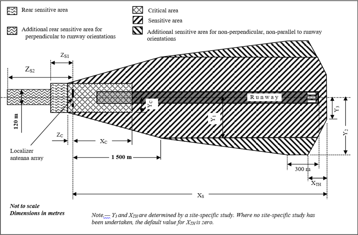
Figure C-3. Example of localizer critical and sensitive area dimensions (values in associated Table C-1 below)
