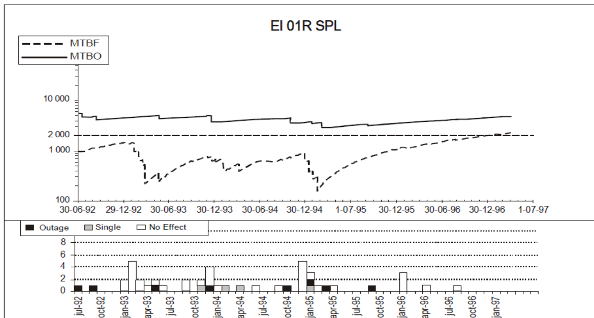
Figure G-35B. Example outage record for MLS elevation facility
