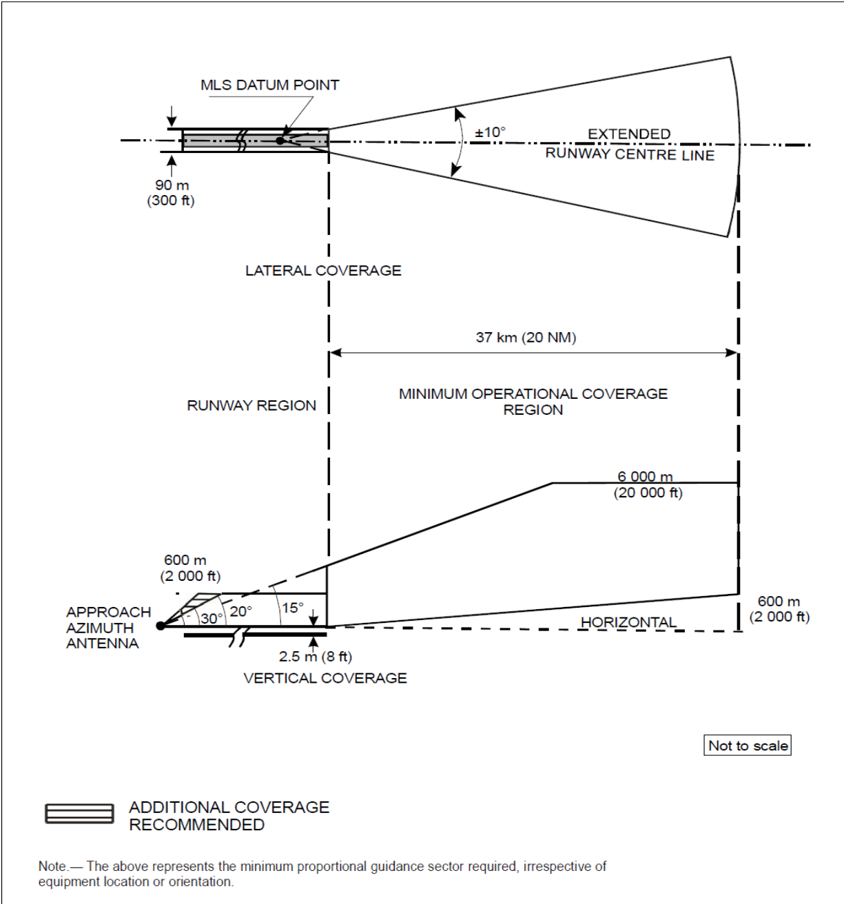
Figure G-5B. Azimuth runway region coverage and minimum operational coverage region
