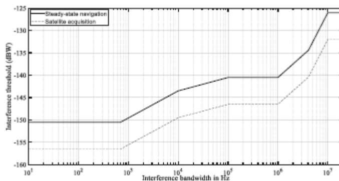
Figure FIG-08A. Interference thresholds versus bandwidth for BDS B1I receiver
