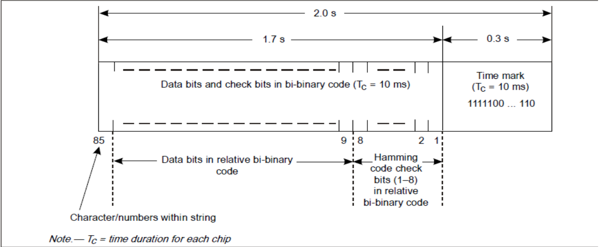
Figure B-10. Data string structure
