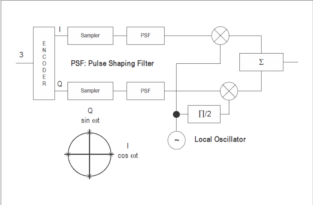
Figure B-19. Example data modulation
