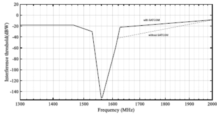
Figure FIG-04A. CW interference thresholds for BDS BII receivers in steady-state navigation
