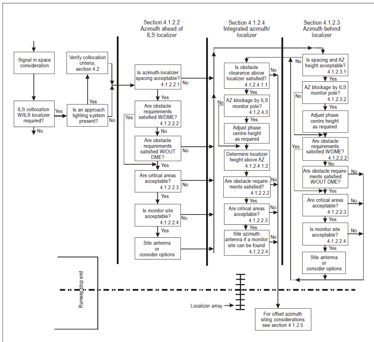
Figure G-20. Azimuth/localizer logic flow diagram
