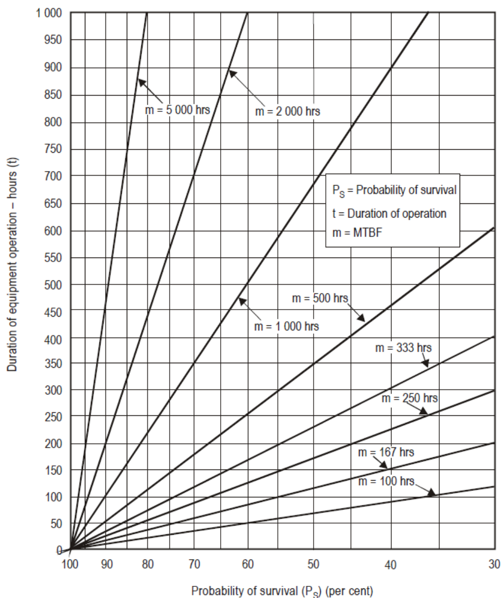
Figure F-1. Plot of P_s = 100 e^{-t/m}
