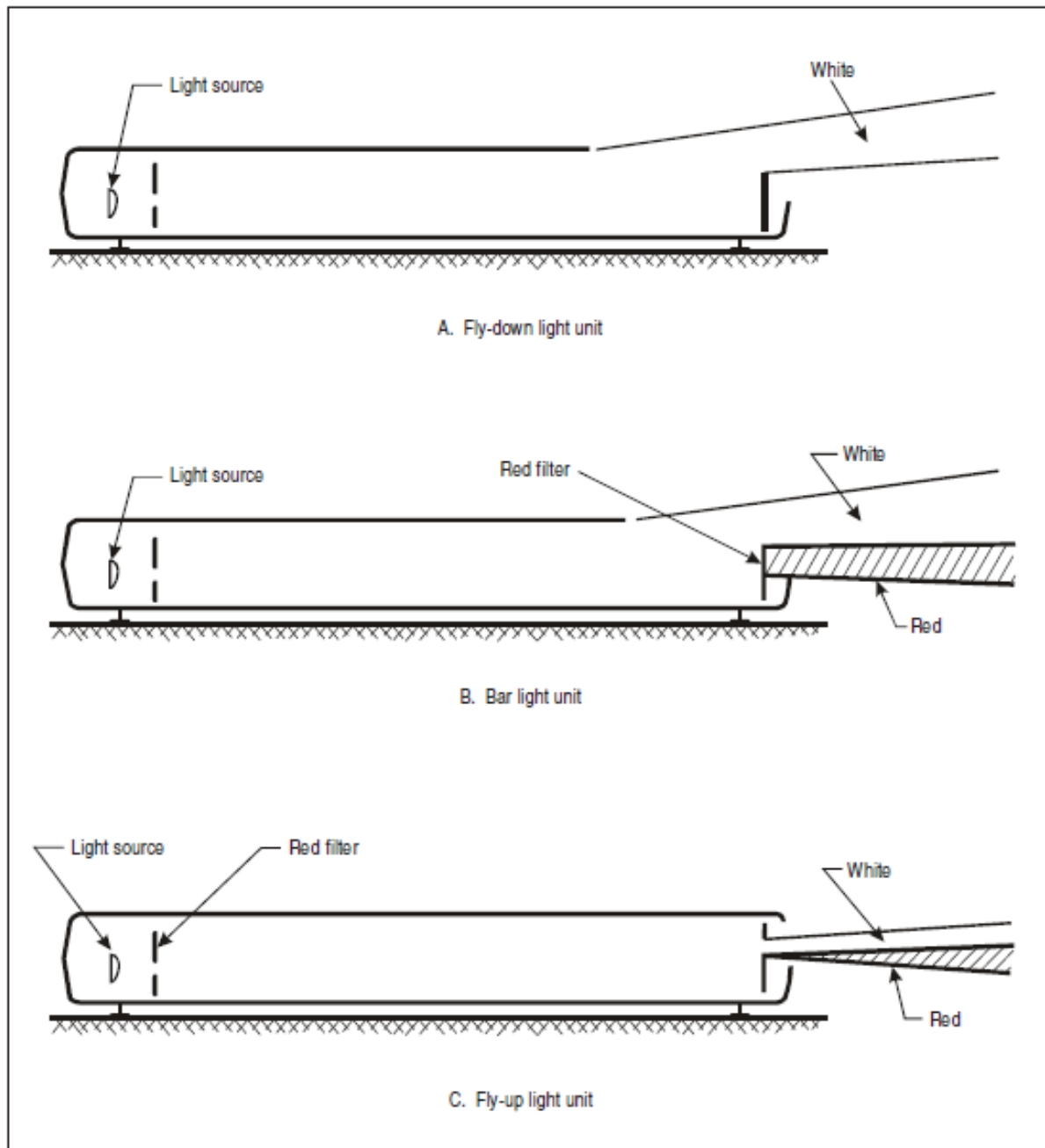
Figure 8-4. T-VASIS light units (blade type)
