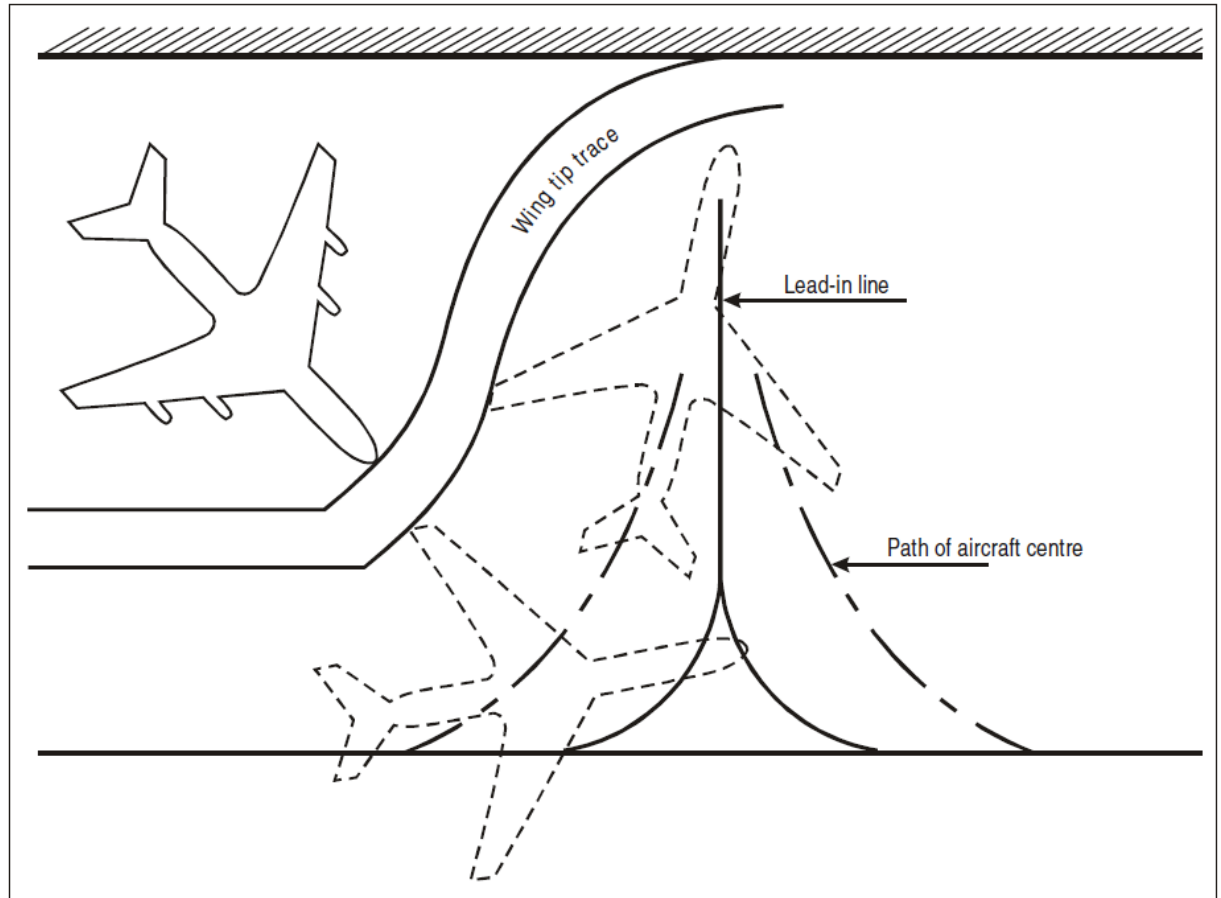
Figure 2-2. Simple nose-wheel lead-in line
