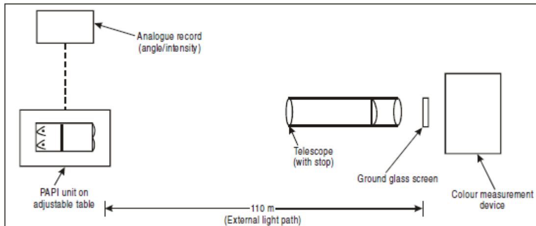
Figure 8-10. Layout of test laboratory
