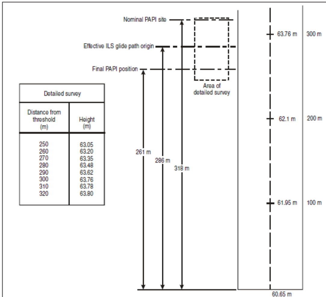
Figure 8-12. Survey data
