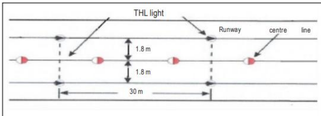
Figure 19-8. Position of lights on THL rows
