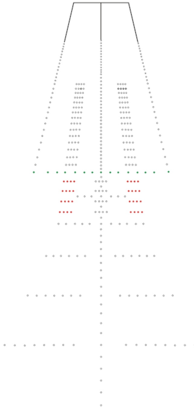
Figure 16-2. Approach and runway lighting, reduced pattern
