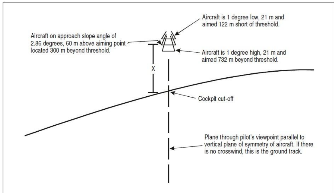
Figure 1-4. Height and aiming errors as they appear when only the runway is visible and there is no horizon
