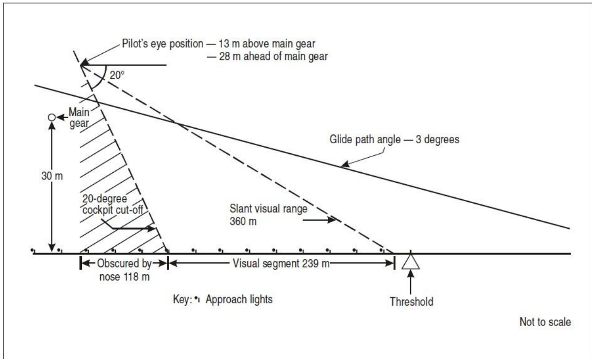
Figure 1-2. Visual segment from a large-bodied jet aircraft
