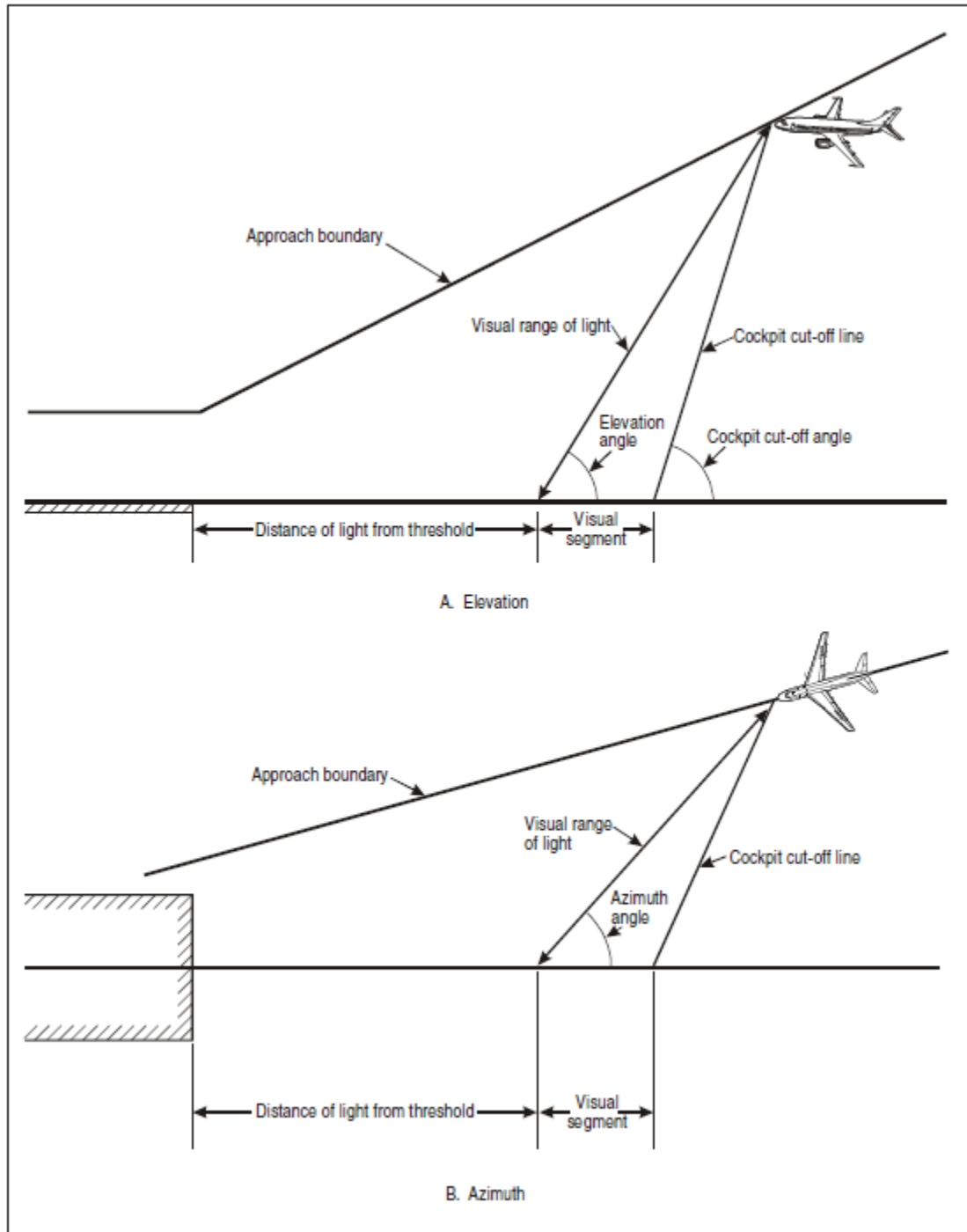
Figure 4-1. Visual segment geometry
