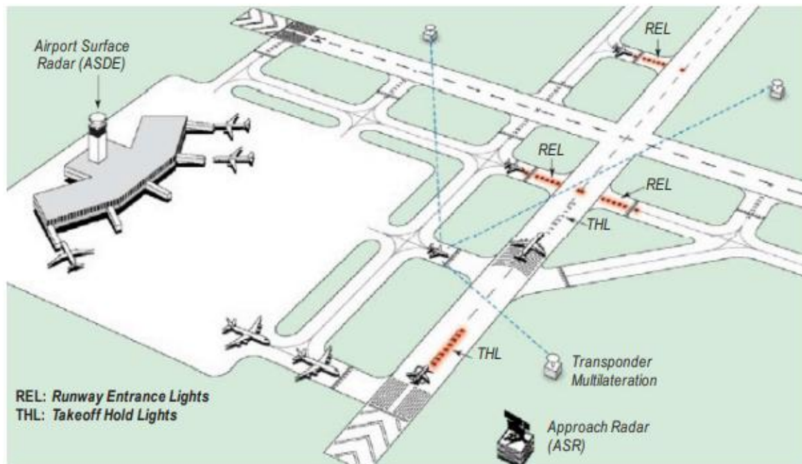
Figure 19-1. Runway Status Lights (RWSL) Source: www.RWSL.net
