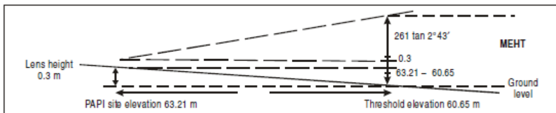
Figure 8-13. MEHT back-check
