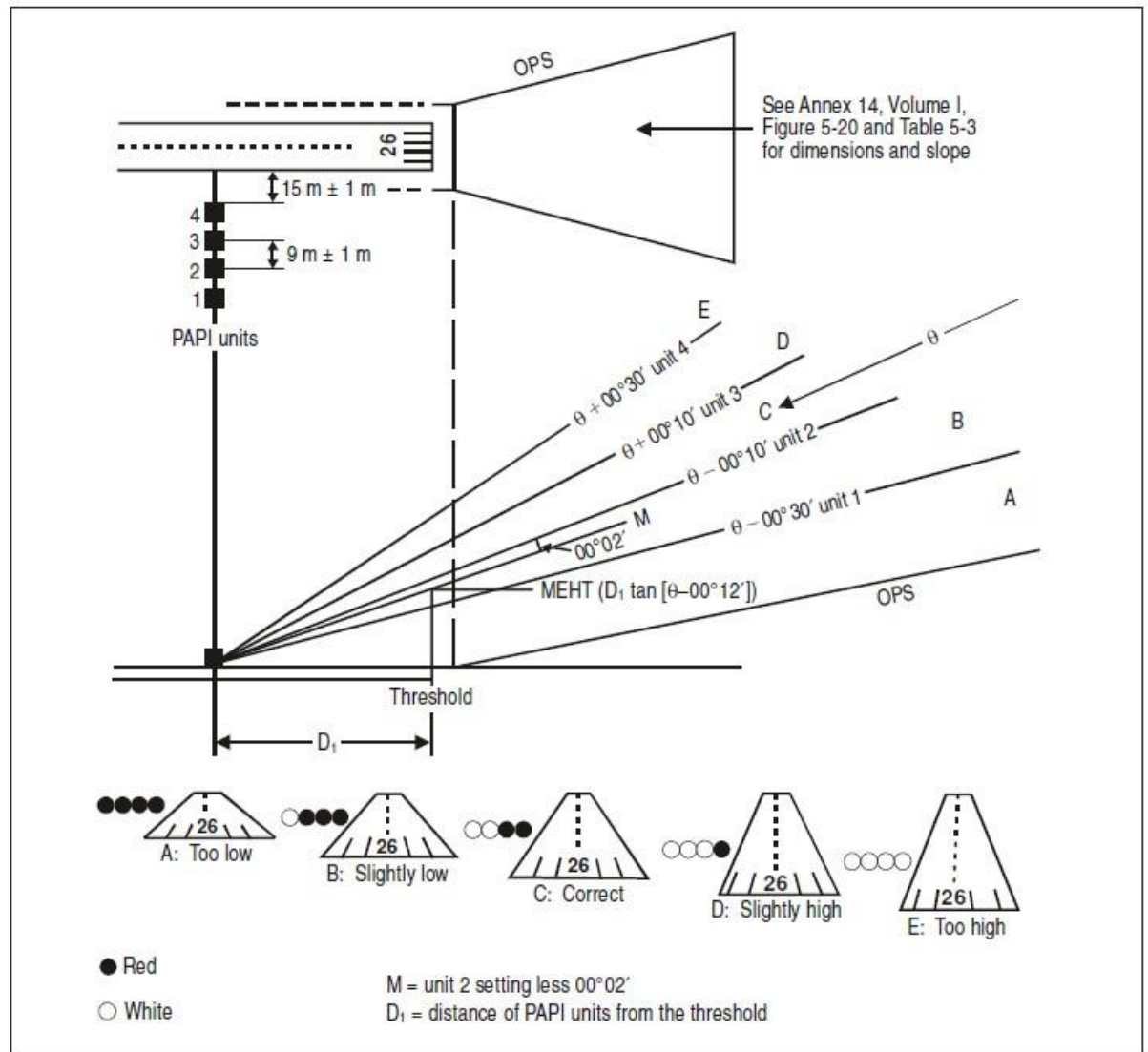
Figure 8-6. The arrangement of the PAPI units and the resulting display
