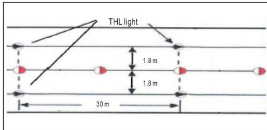
Figure 19-9. Position of lights on THL rows
