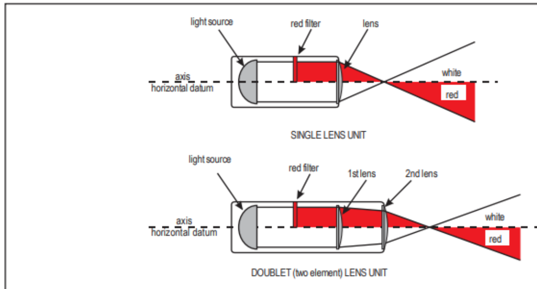
Figure 8-9. PAPI light unit
