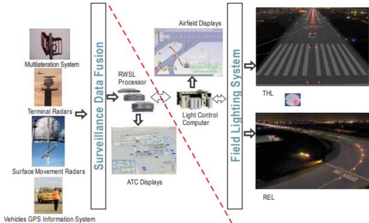
Figure 19-2. Types of surveillance systems providing feeds to RWSL System
