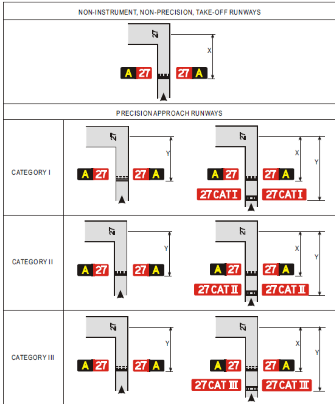
Figure 11-3. Examples of sign positions at taxiway/runway intersections
