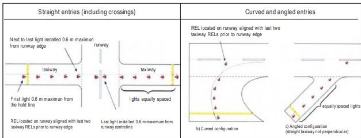
Figure 19-4. Layout of RELs
