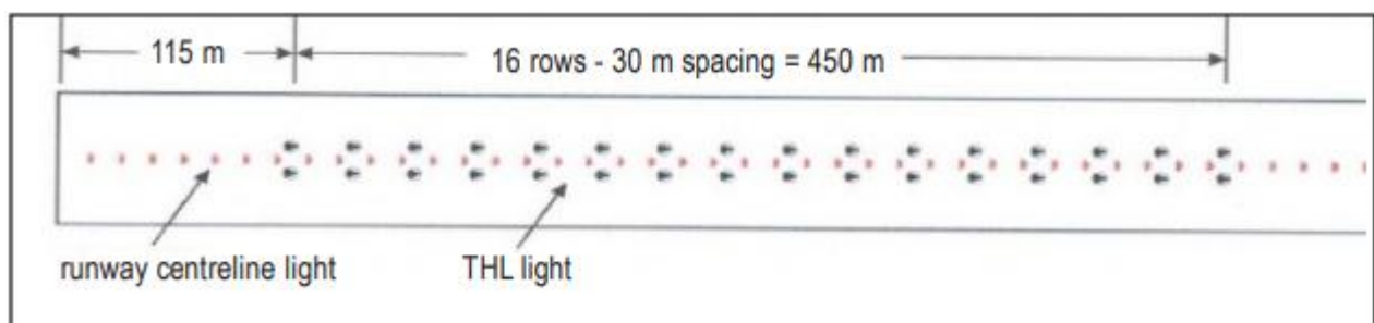
Figure 19-6. Layout of THLs
