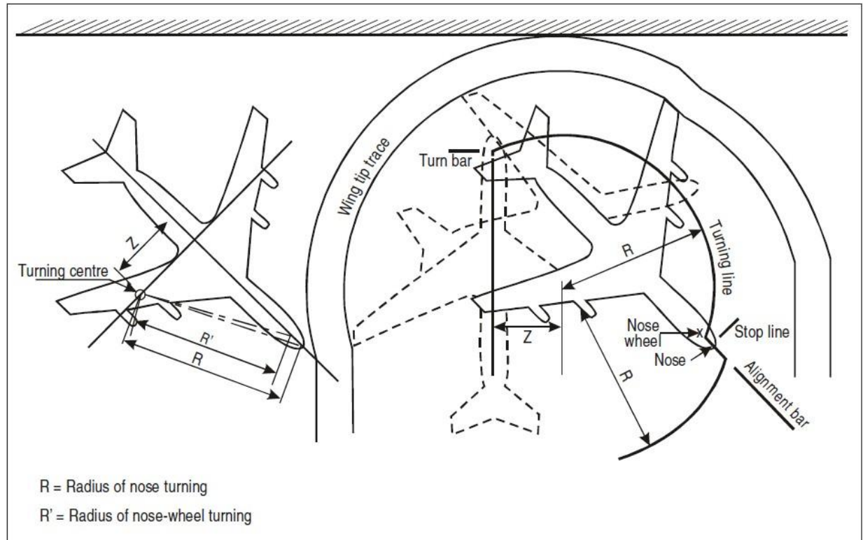
Figure 2-5. Turning line and reference bars
