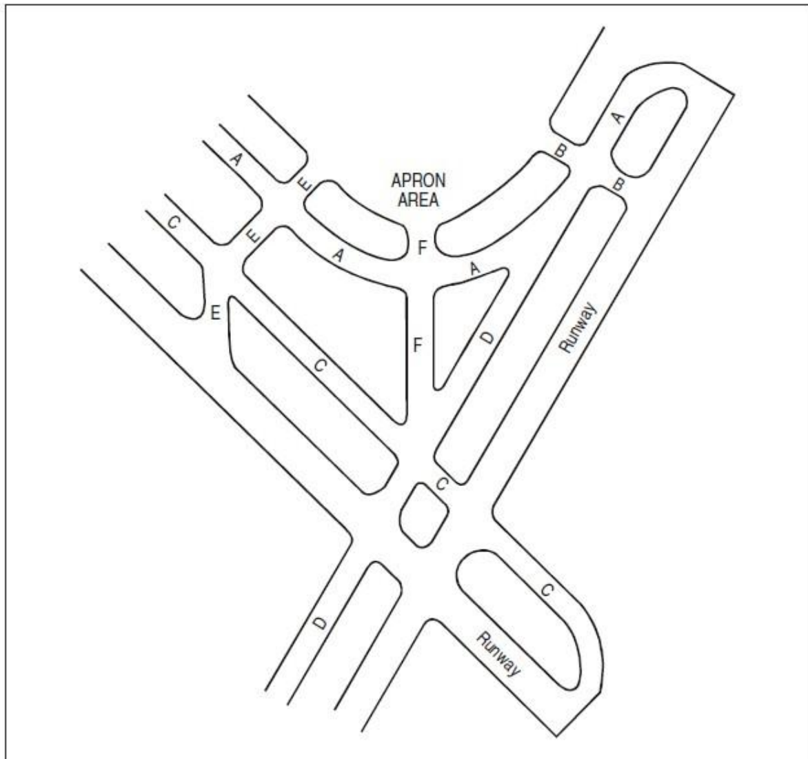
Figure 11-6. Assignment of letters to taxiways
