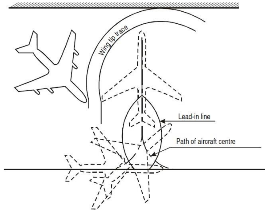
Figure 2-3. Offset nose-wheel lead-in line
