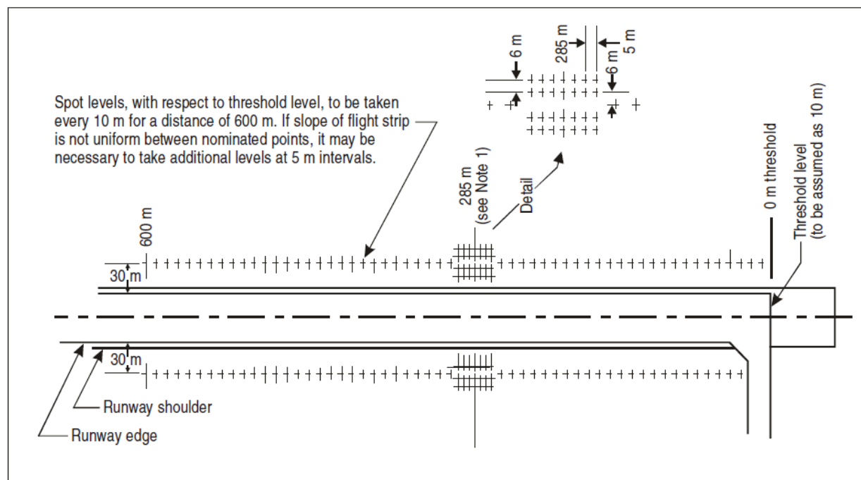
Figure 8-1. T-VASIS location survey
