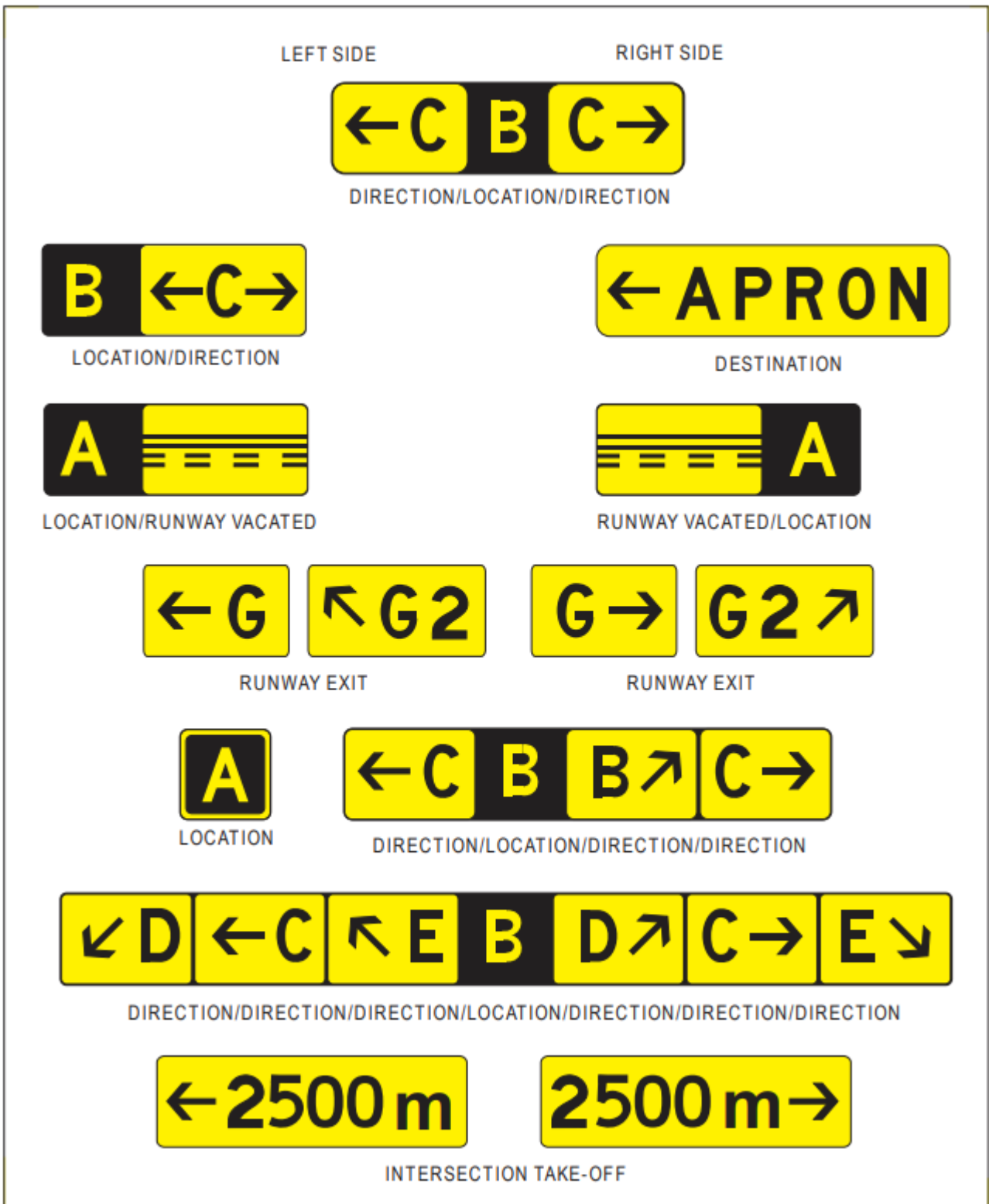
Figure 11-5. Information signs
