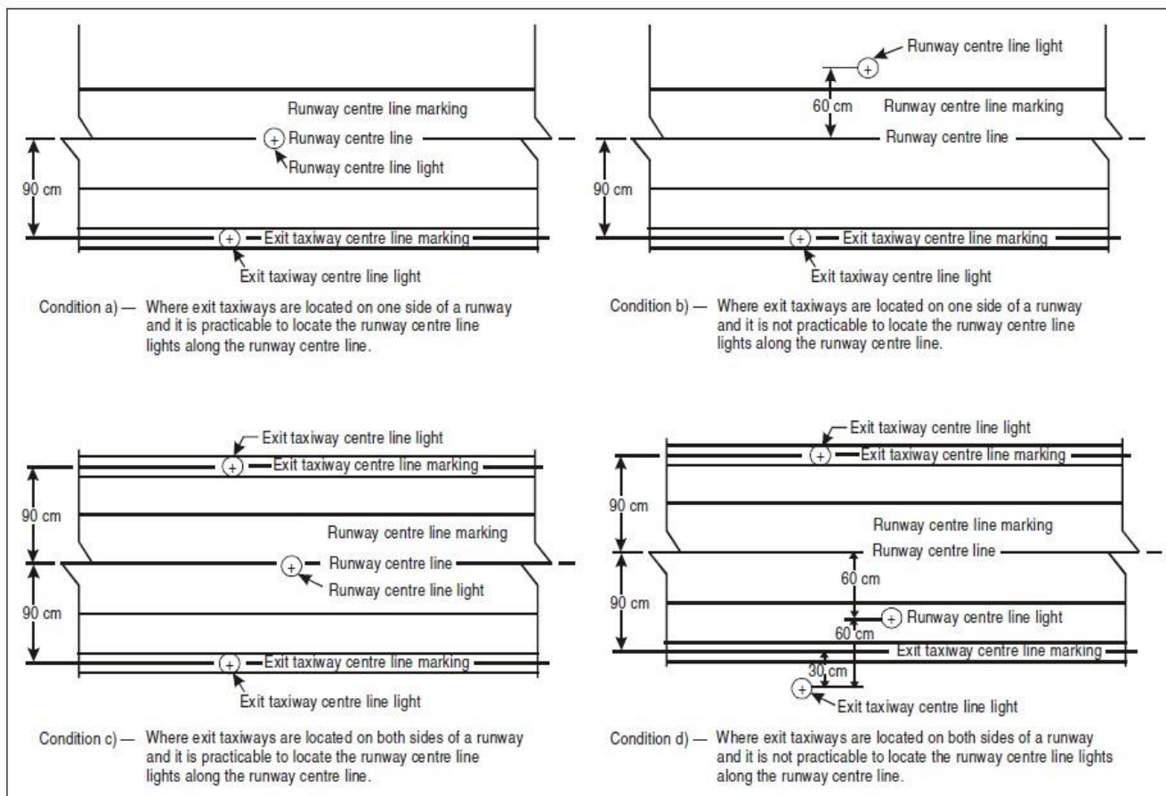
Figure 9-2. Marking and lighting of runway/taxiway intersections
