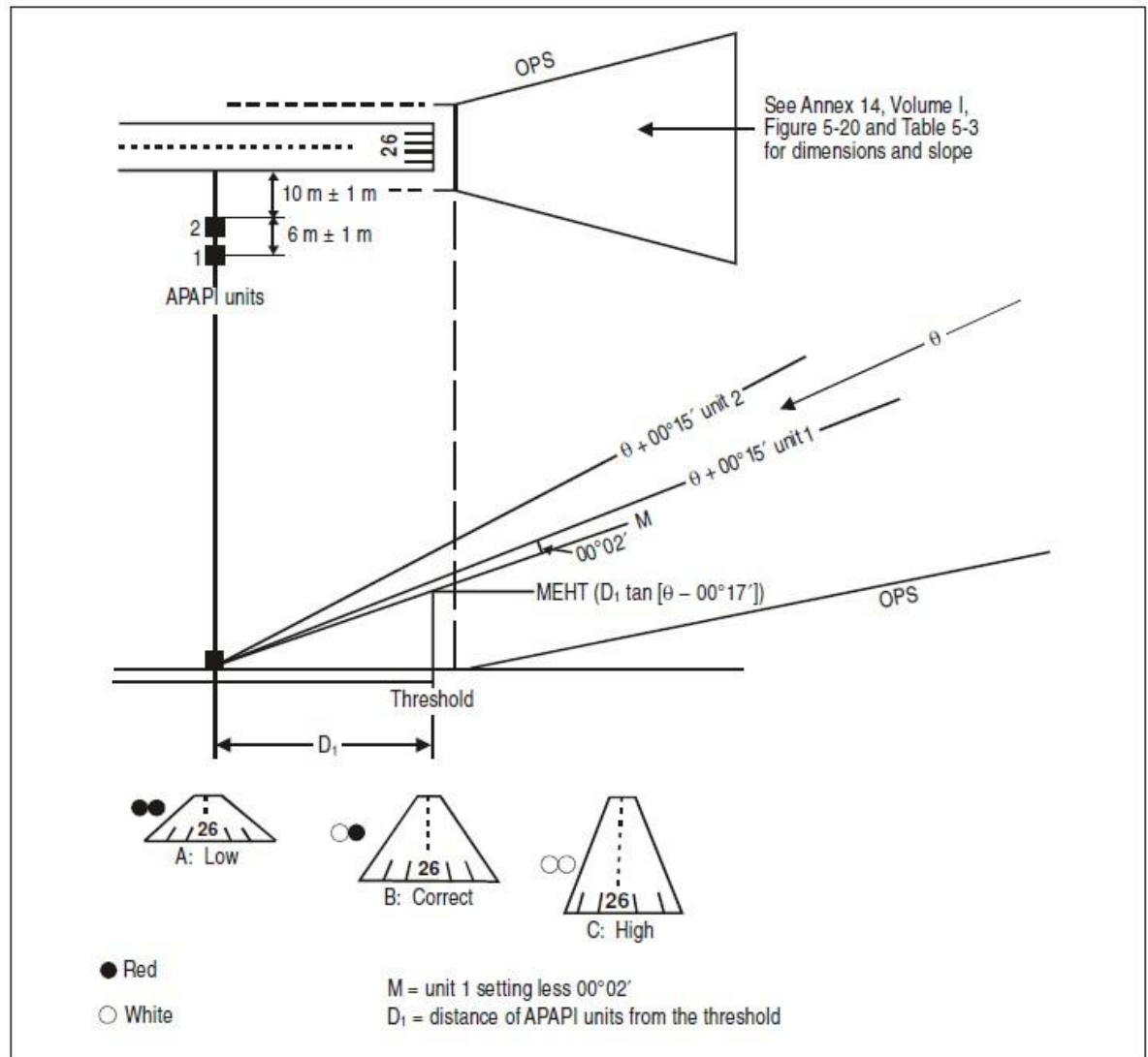
Figure 8-7. The arrangement of the APAPI units and the resulting display
