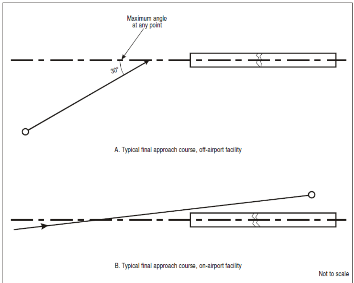
Figure 1-5. Examples of straight-in landings, non-precision aids
