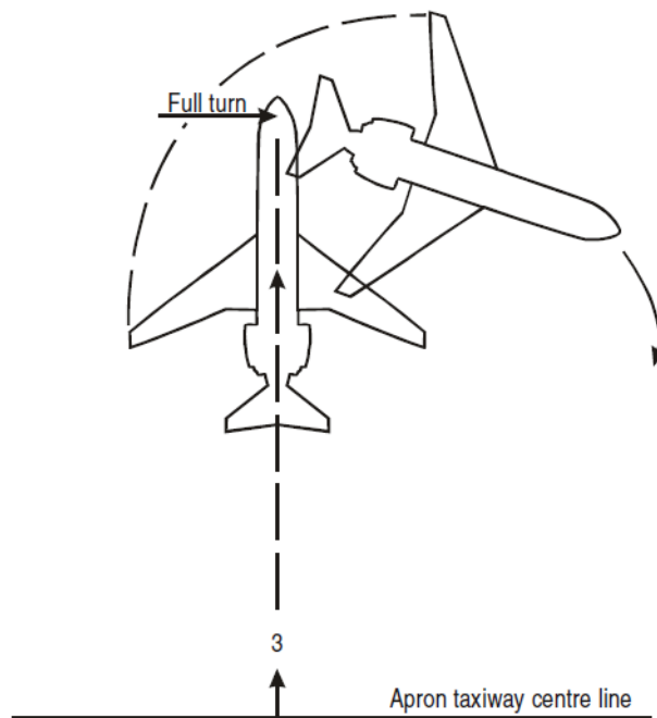
Figure 2-4. Straight lead-in line
