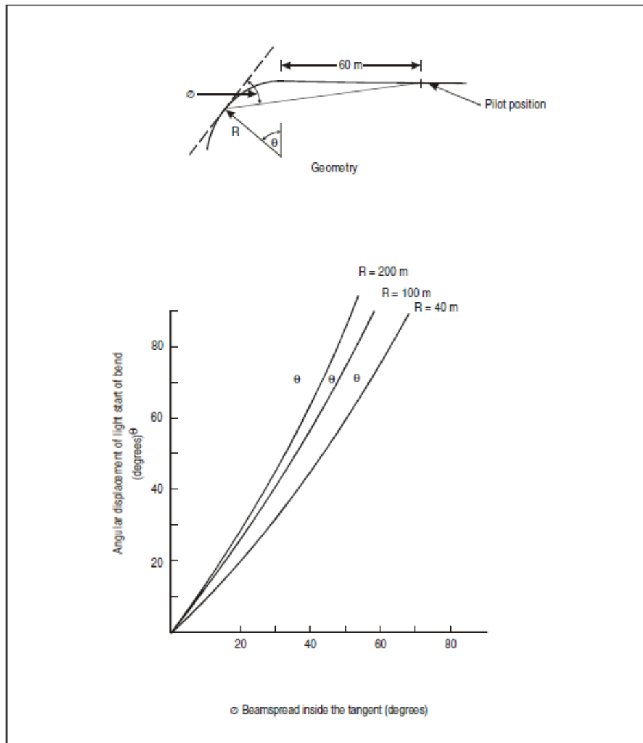
Figure 4-2. Taxiway lighting geometry
