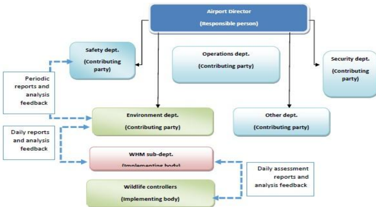
Figure 2: Organisational Chart
