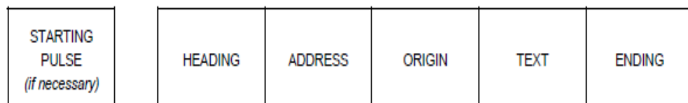
Figure 4-2. Form of transmission — teletypewriter operation (see 4.4.10.1.2)
