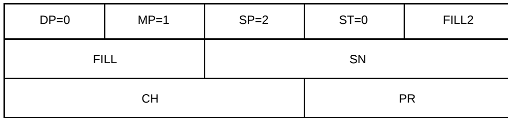
Figure 5-15. RECEIVE READY packet
