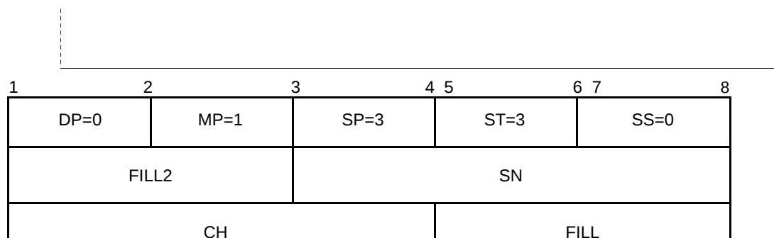
Figure 5-13. INTERRUPT CONFIRMATION packet
