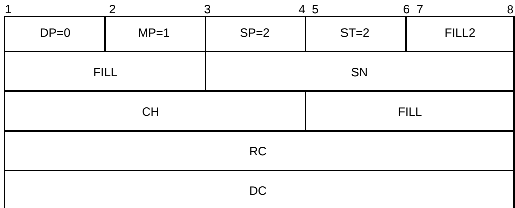
Figure 5-17. RESET REQUEST packet
