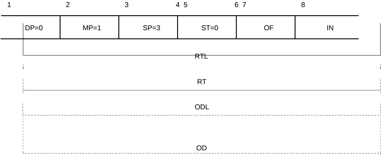
Figure 5-19. ROUTE packet
