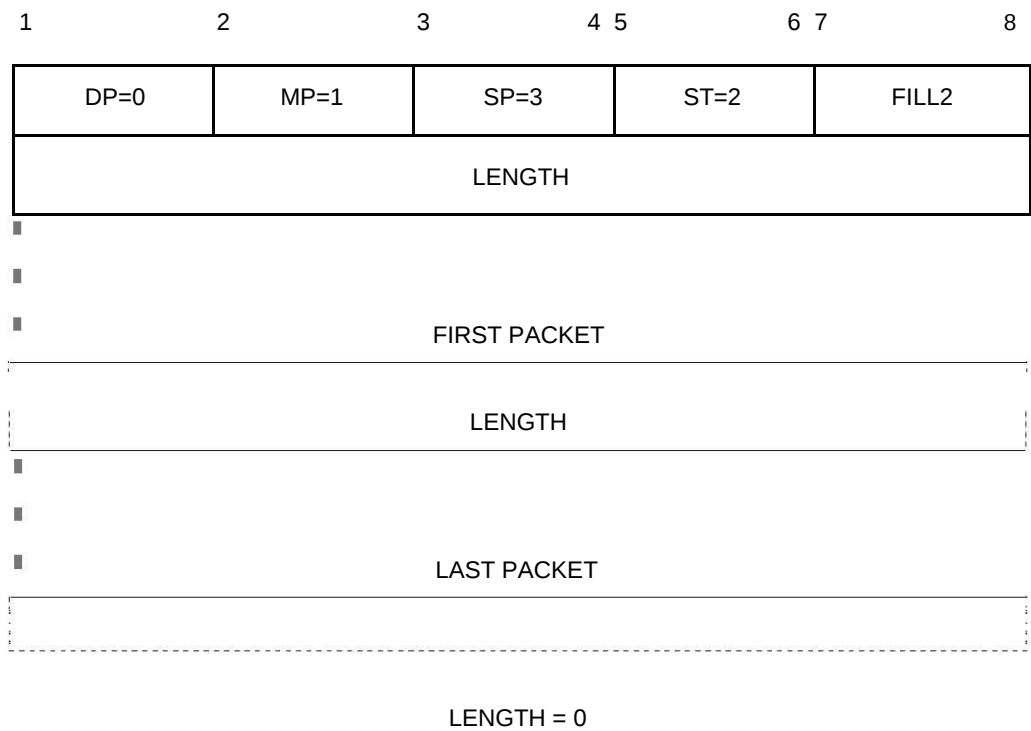
Figure 5-20. MULTIPLEX packet
