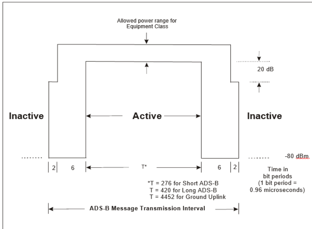
Figure 12-2. Time/amplitude profile of UAT message transmission
