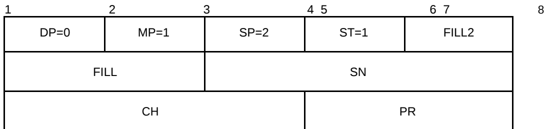
Figure 5-16. RECEIVE NOT READY packet
