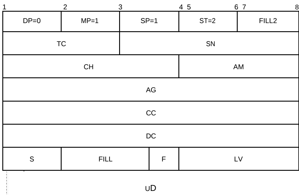
Figure 5-7. CLEAR REQUEST by ADLP packet
