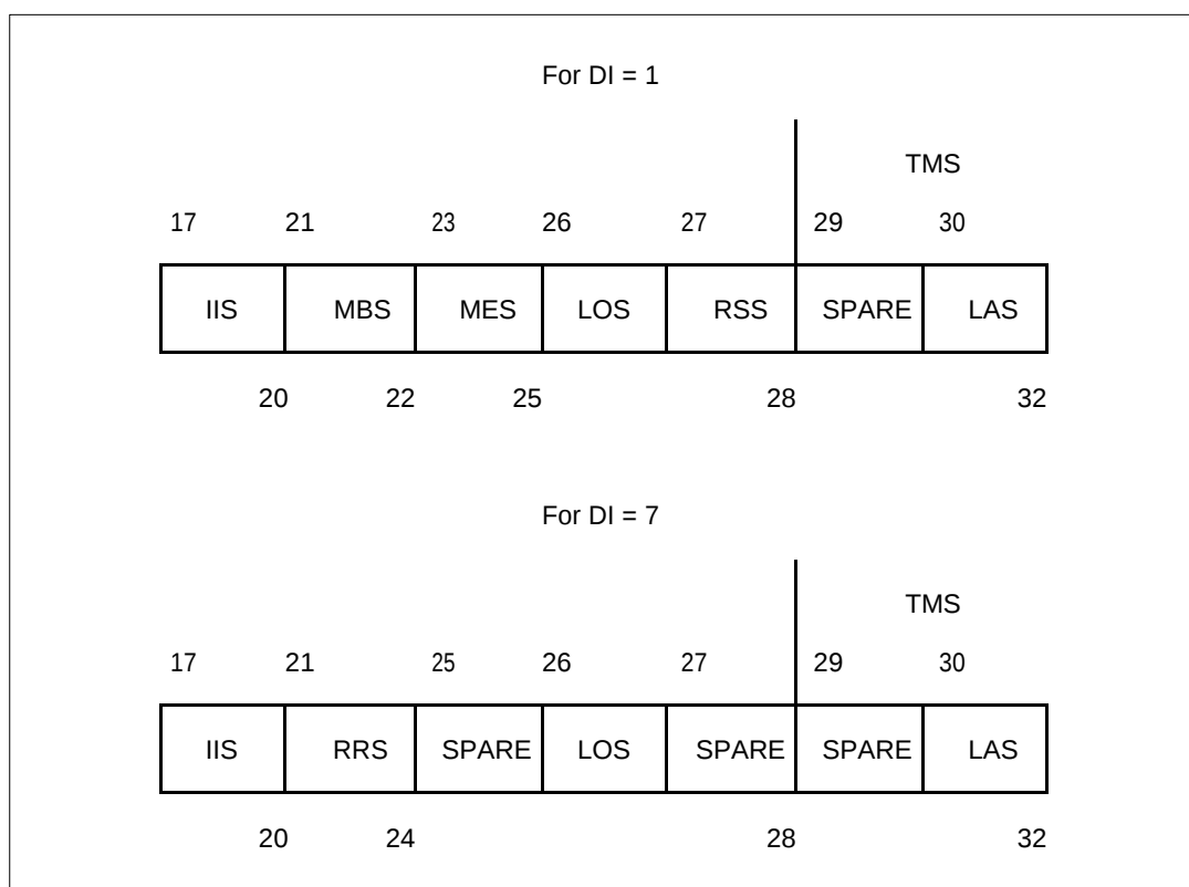
Figure 5-1. The SD field structure
