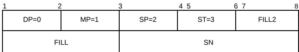
Figure 5-18. RESET CONFIRMATION packet
