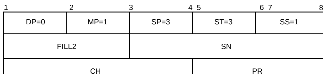
Figure 5-14. REJECT packet
