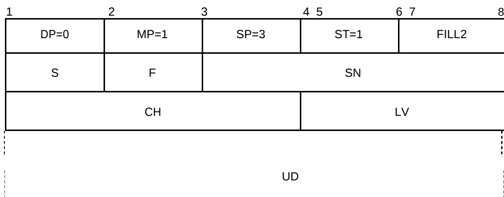
Figure 5-12. INTERRUPT packet
