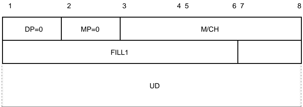
Figure 5-21. SHORT FORM MSP packet
