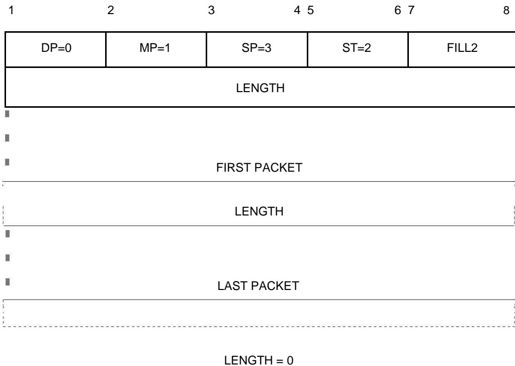
Figure 5-20. MULTIPLEX packet
