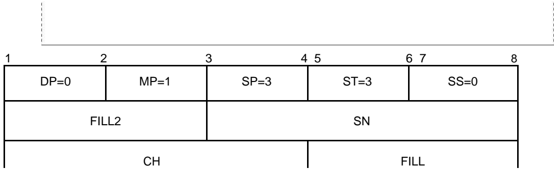
Figure 5-13. INTERRUPT CONFIRMATION packet
