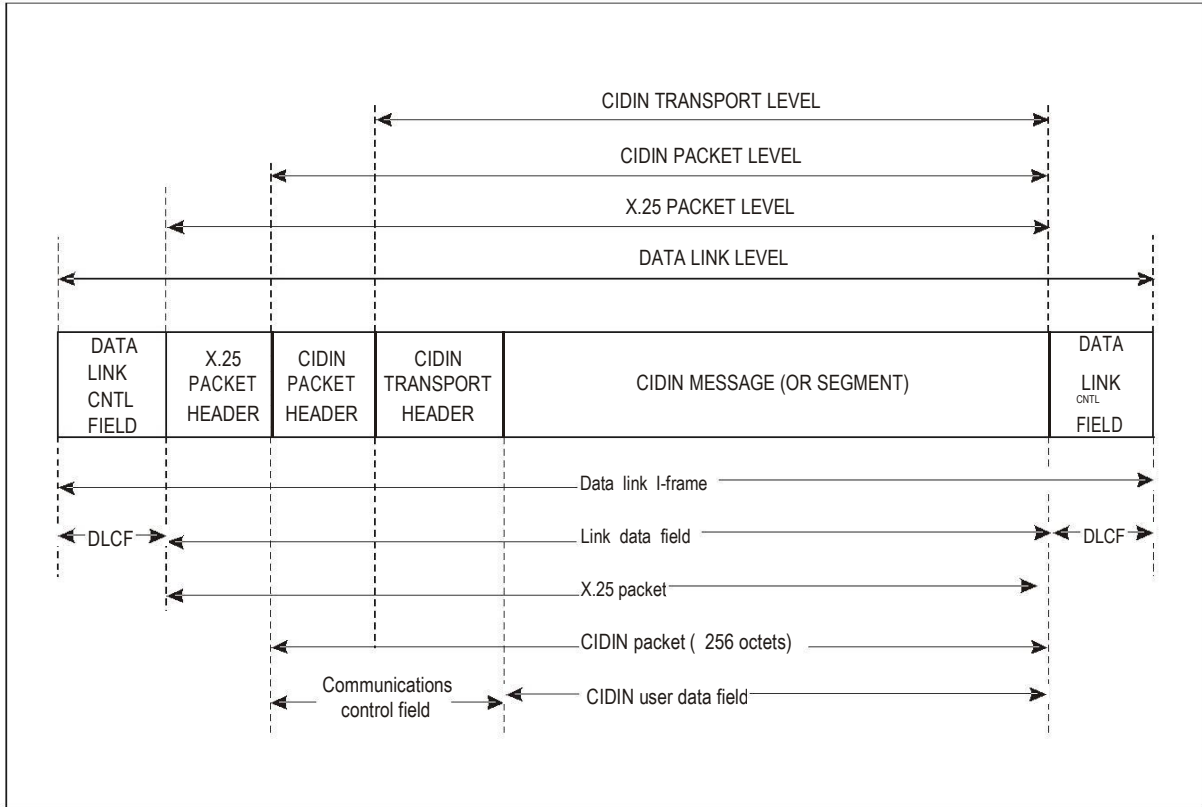
Figure 8-2. CIDIN terminology
