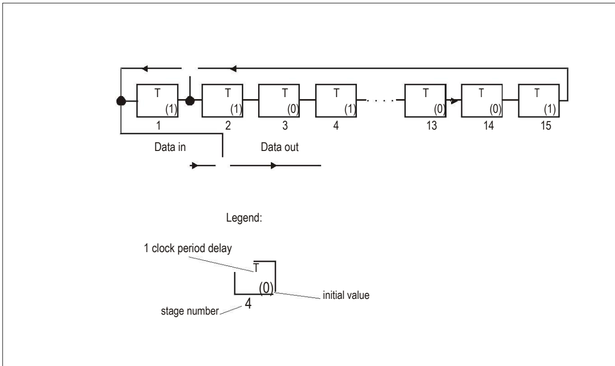
Figure 6-2. PN-generator for bit scrambling sequence
