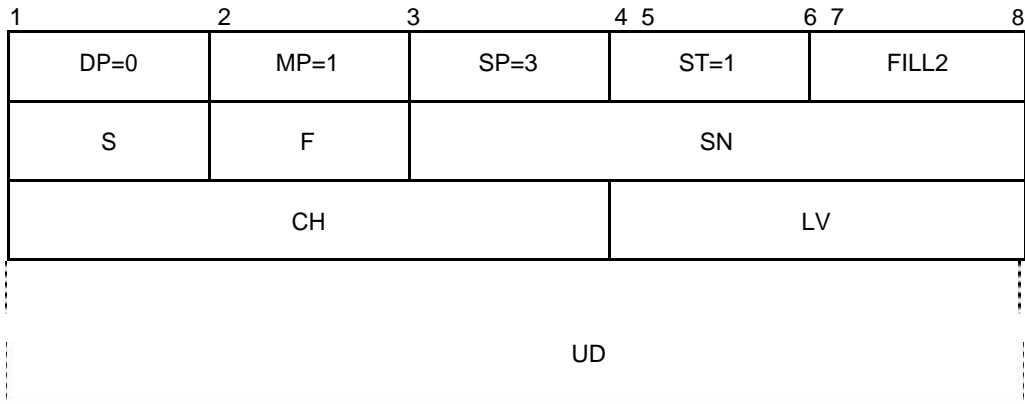
Figure 5-12. INTERRUPT packet
