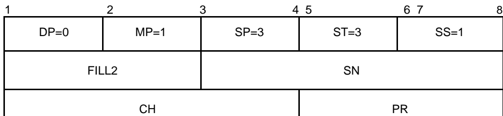
Figure 5-14. REJECT packet
