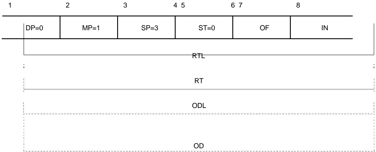
Figure 5-19. ROUTE packet
