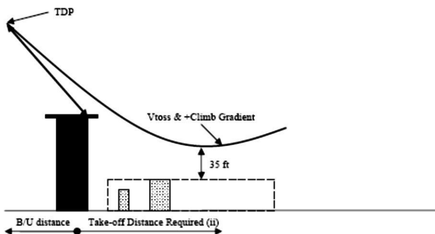
Figure 4: Elevate Helipad take – off
