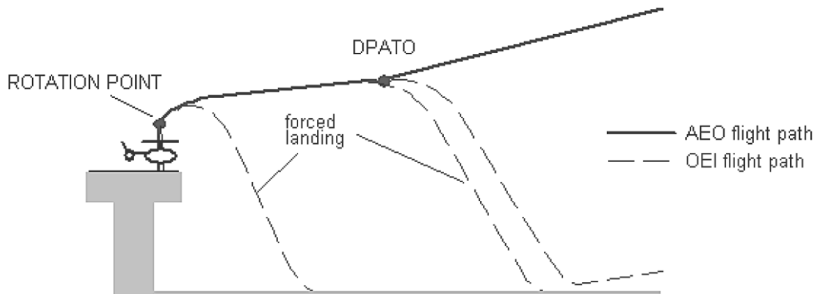
Figure 1: Take-off profile
