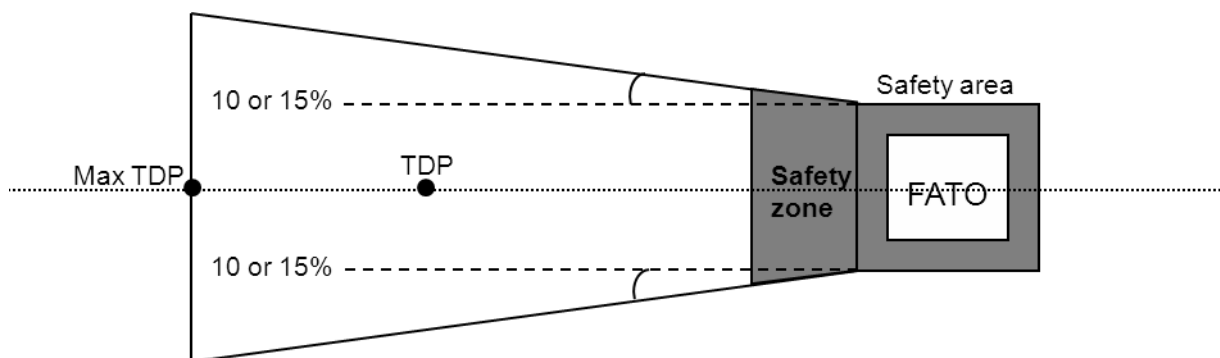
Figure 2: Obstacle accountability
